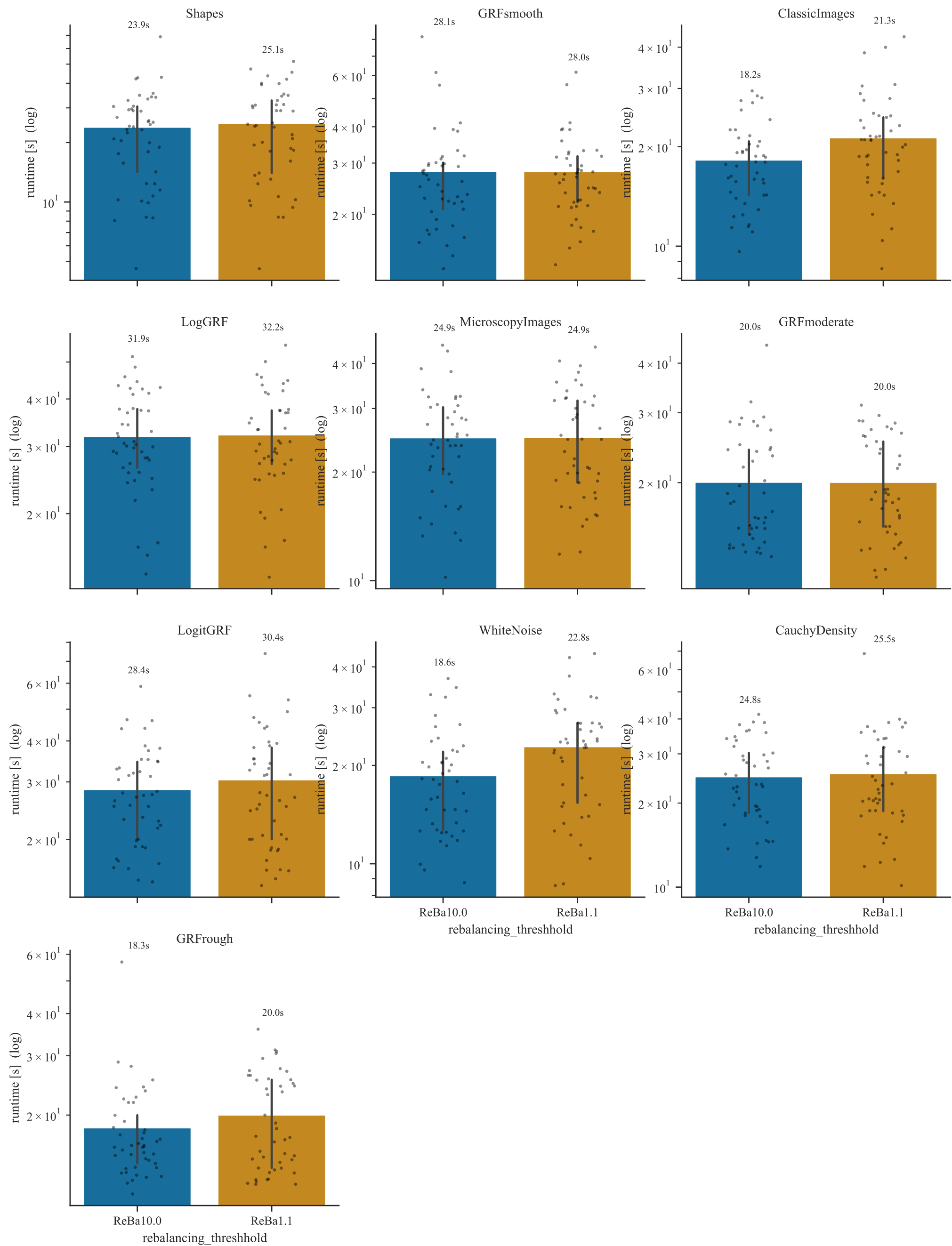
Runtime for different rebalancing_threshold values
