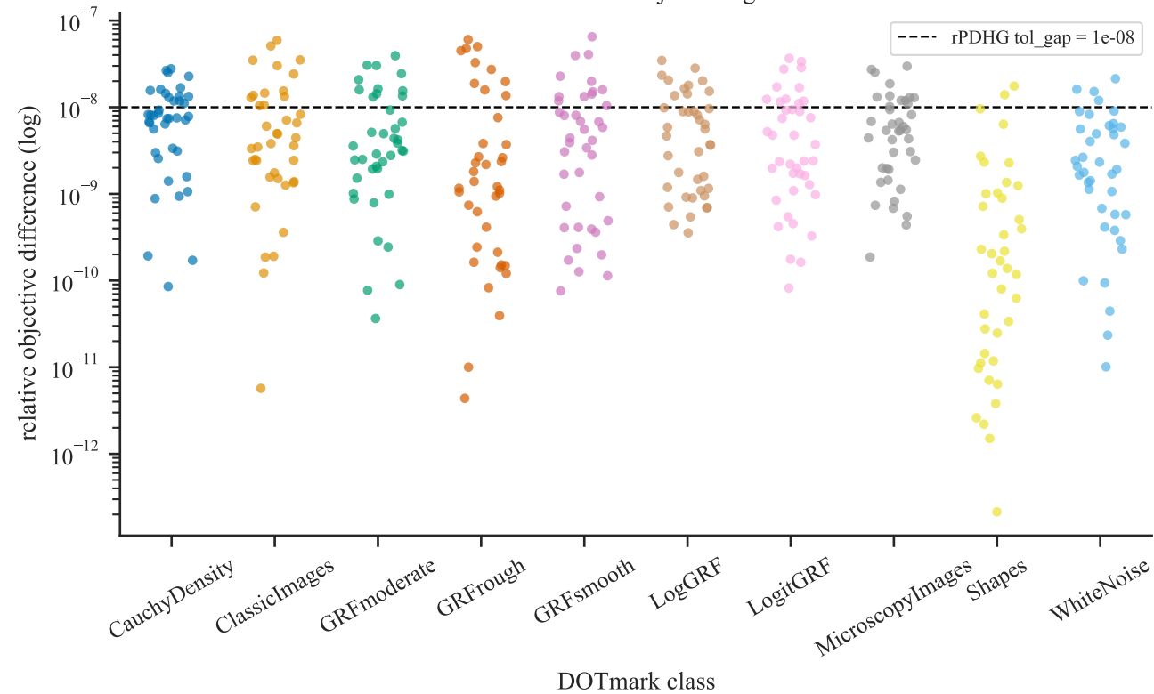
rPDHG vs Gurobi: objective agreement
