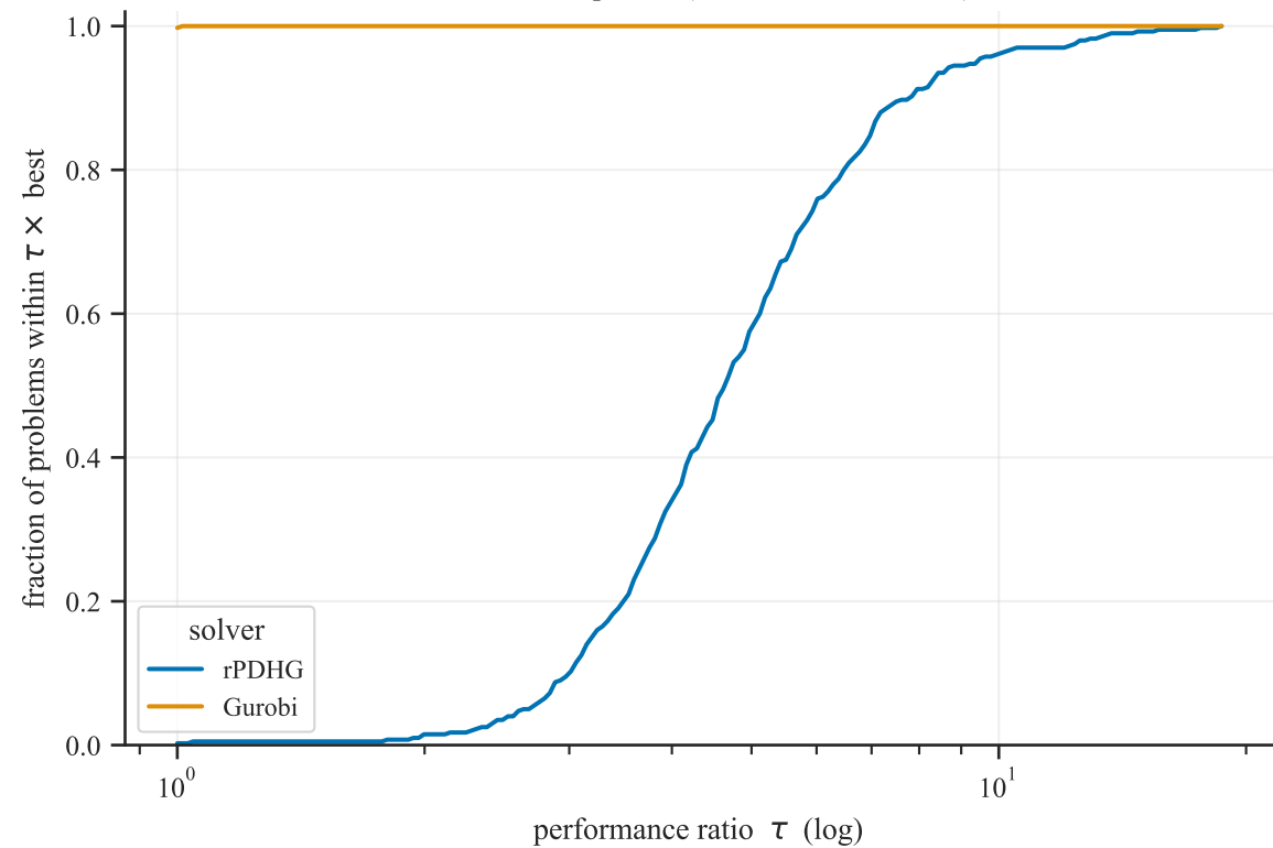
Performance profile (Dolan–Moré, runtime)
