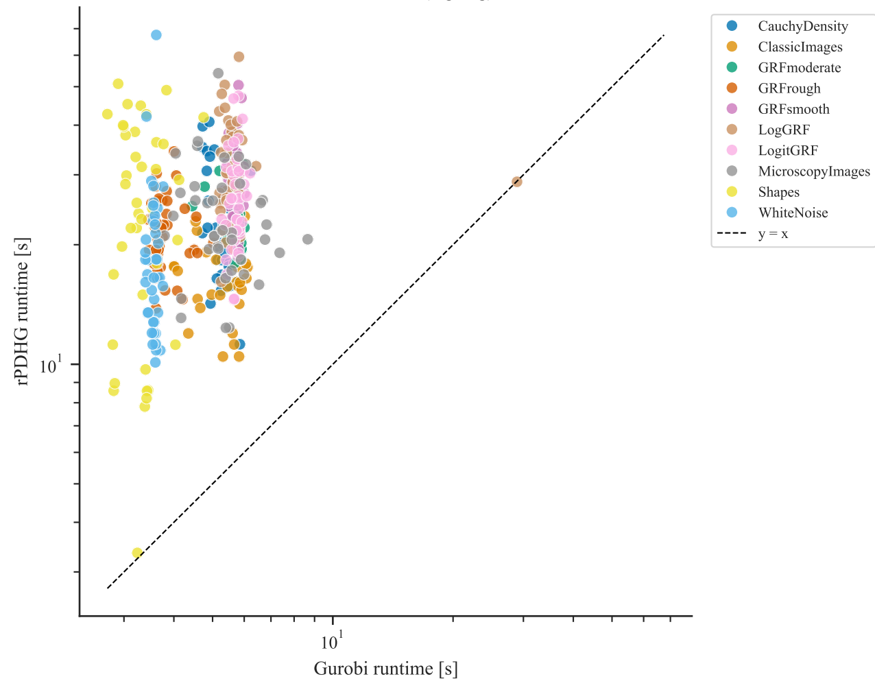
rPDHG vs Gurobi (log-log)
