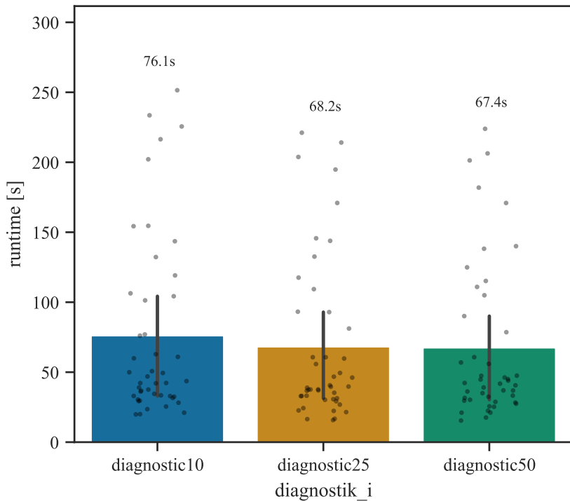
LogGRF: total runtime (no clean trend — iteration-count confound)
