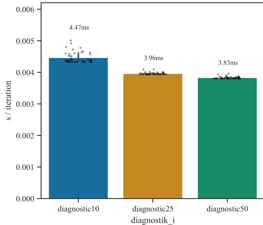
LogGRF: seconds per iteration (isolates sync overhead)
