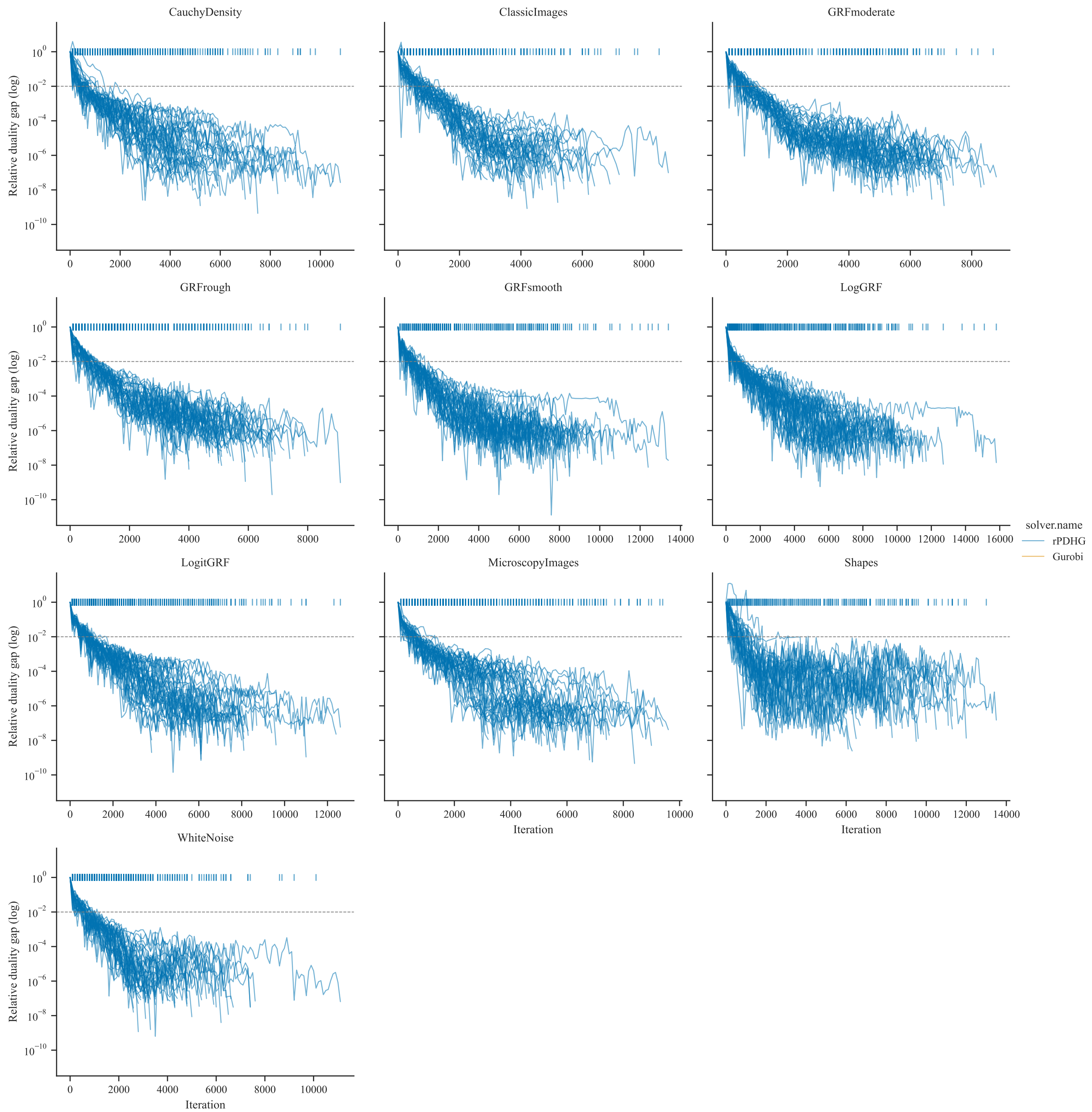
Duality-gap decay vs iterations (adaptive restart)
