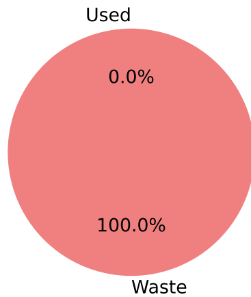
Material Utilization
