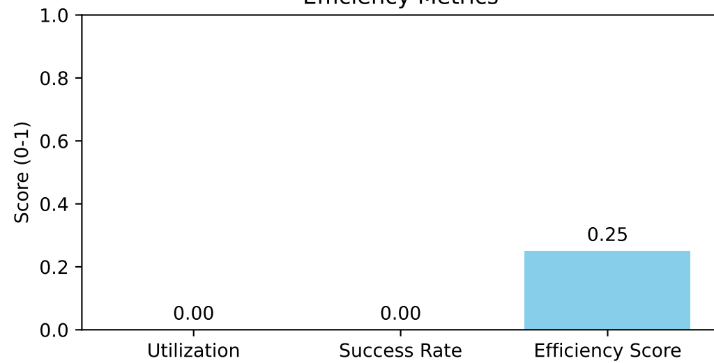
Efficiency Metrics
