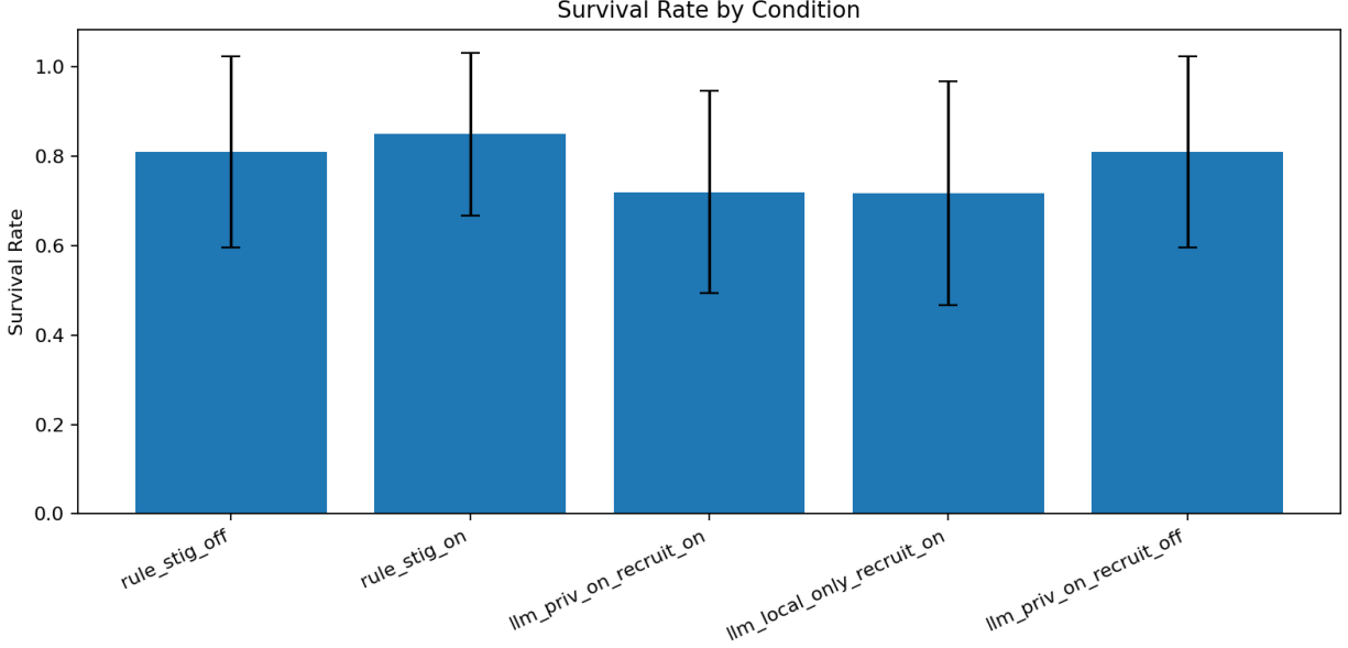
Figure 4: Survival rate by condition. LLM recruitment conditions, llm_priv_on_recruit_on and llm_local_only_recruit_on , show the lowest survival.
