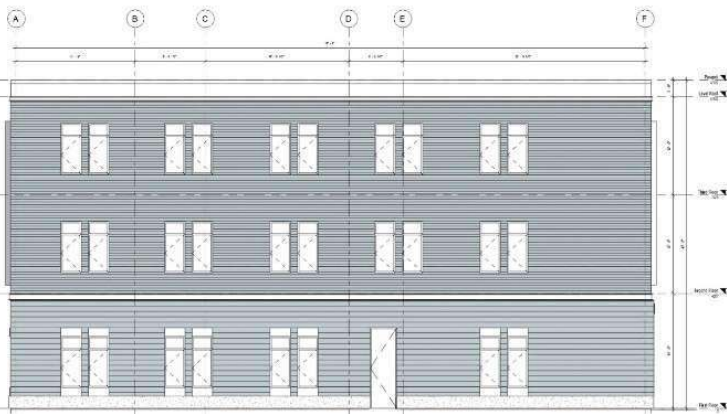
1 South Elevation 1:50
