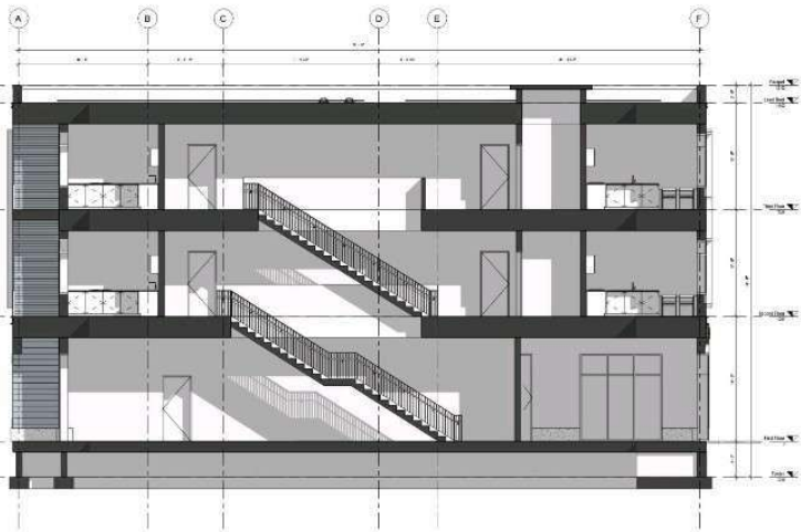
1 Section 1 1:50
