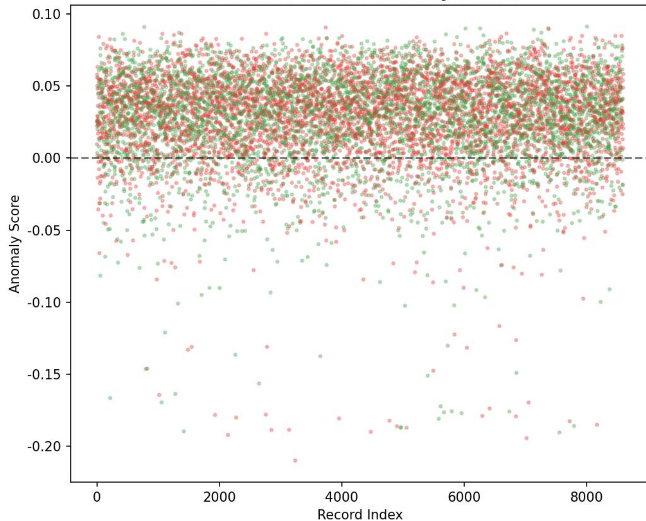
Isolation Forest - Anomaly Scores
