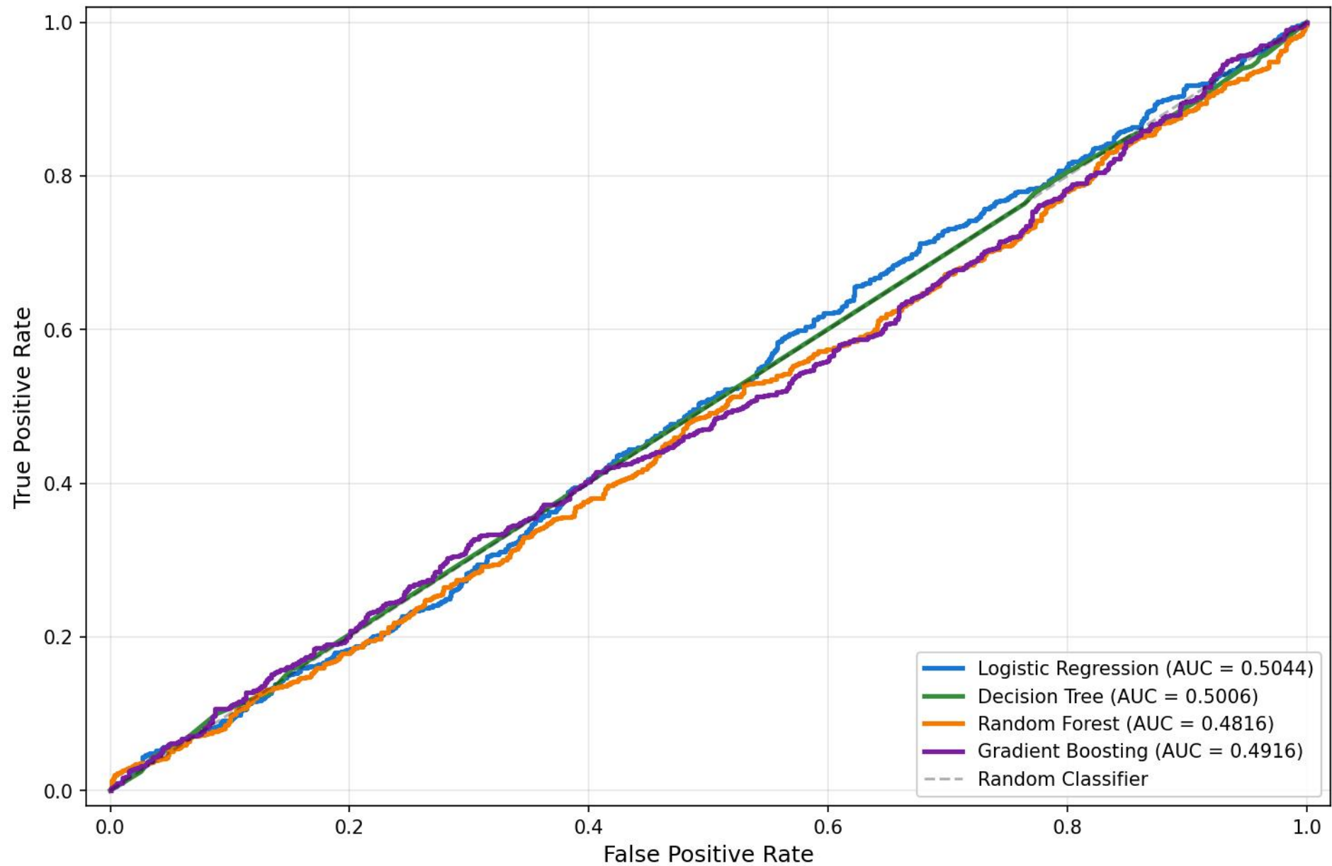
ROC Curves - Model Comparison
