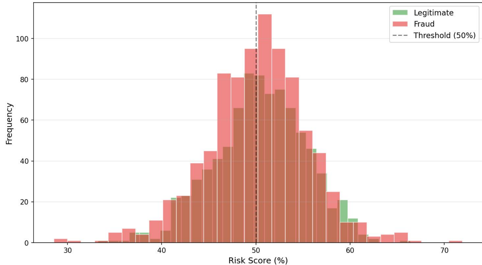
Predicted Risk Score Distribution
