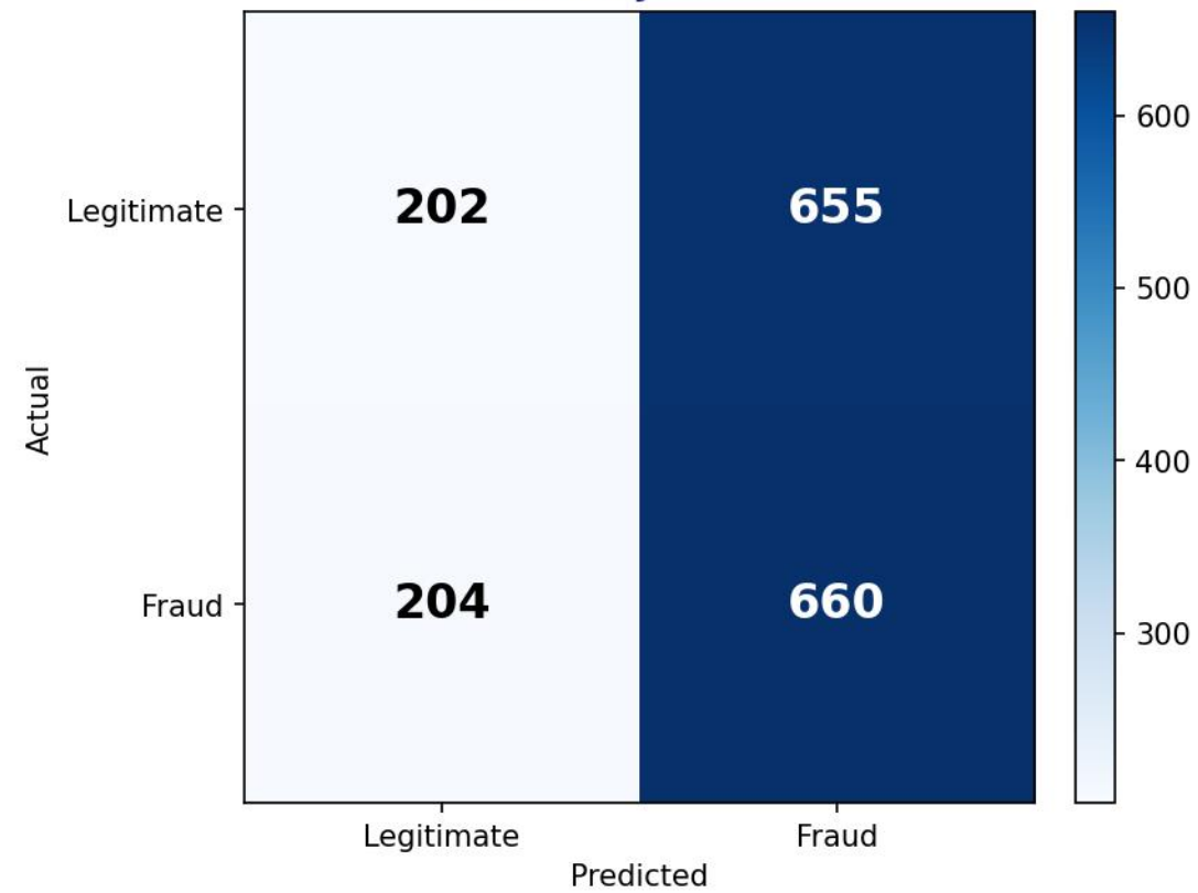
Decision Tree Accuracy: 50.1%
