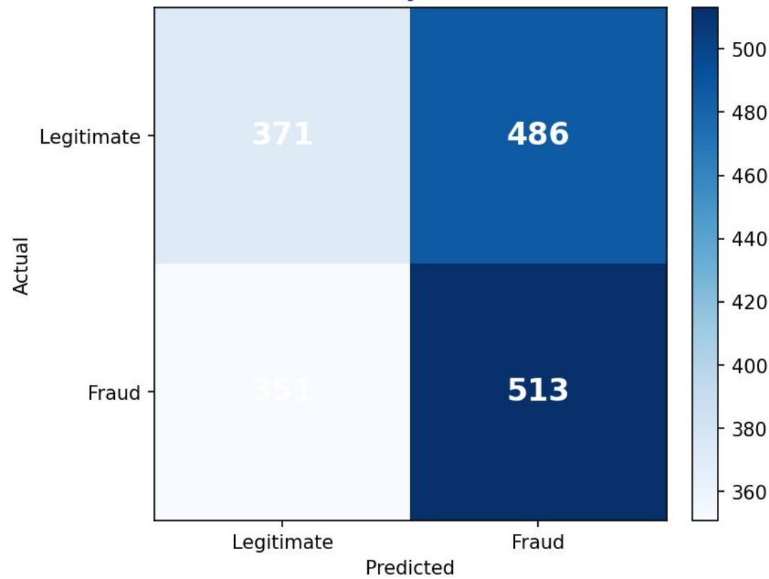
Logistic Regression Accuracy: 51.4%
