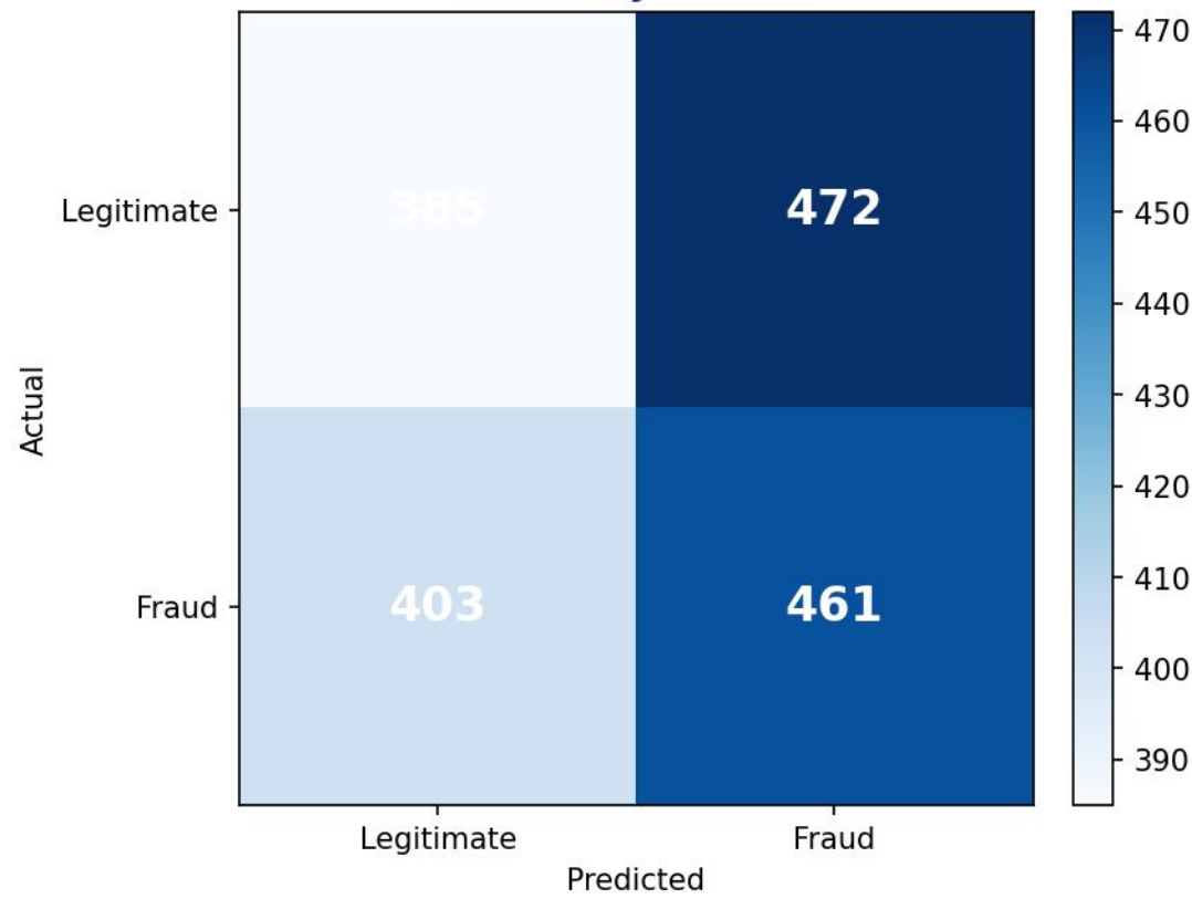
Random Forest Accuracy: 49.2%
