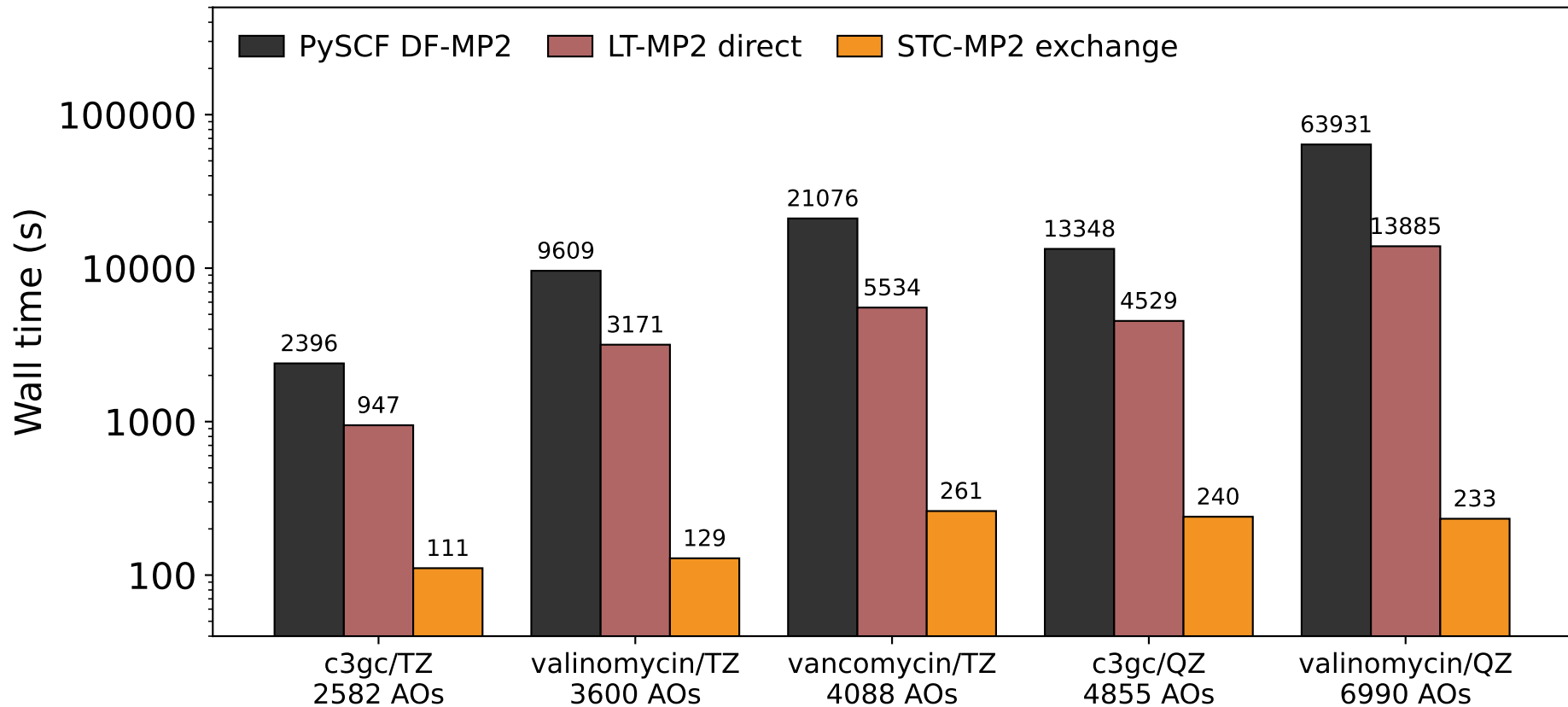
Benchmark on five realistic molecules
