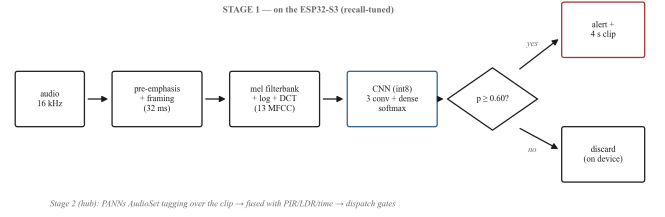
Fig. 3. Stage-1 signal chain on the sensing node: pre-emphasis, windowing, mel filterbank, DCT-II cepstrum, and the quantized CNN classifier, all within the sub-50 ms frame budget.
