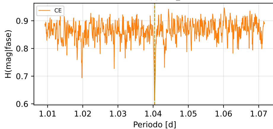
Conditional Entropy (CE_min=0.599)
