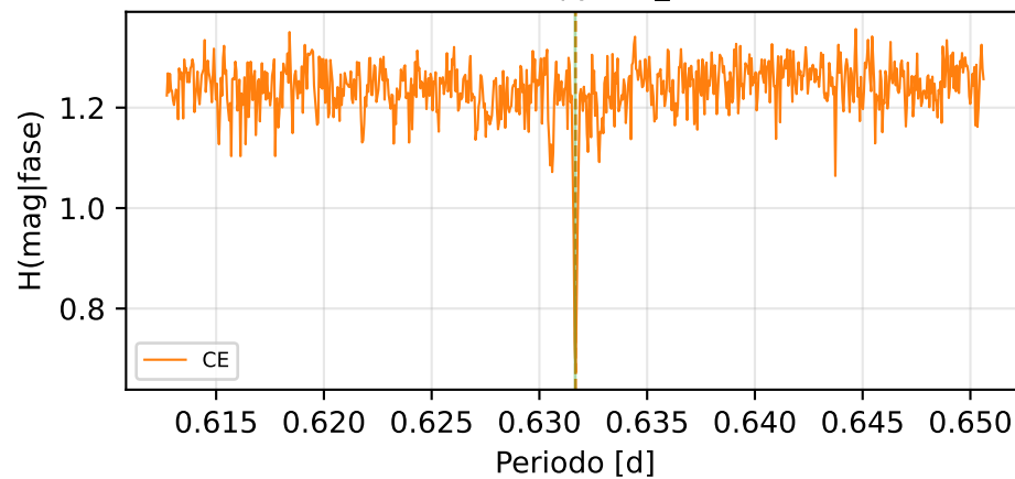
Conditional Entropy (CE_min=0.643)
