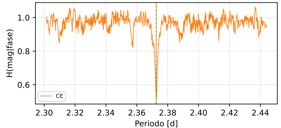
Conditional Entropy (CE_min=0.520)
