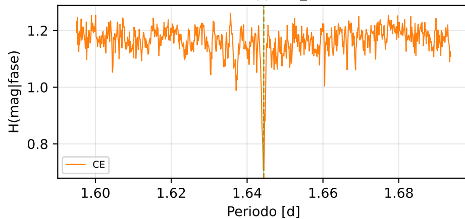
Conditional Entropy (CE_min=0.677)
