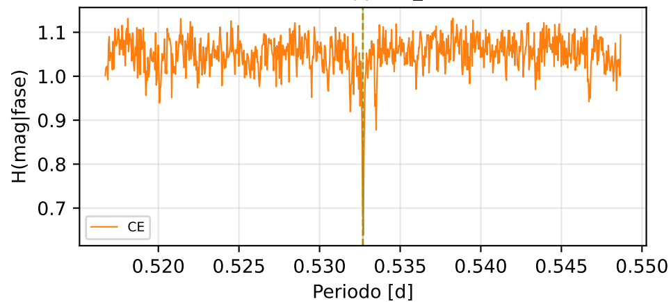
Conditional Entropy (CE_min=0.630)
