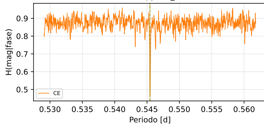
Conditional Entropy (CE_min=0.406)
