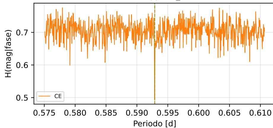
Conditional Entropy (CE_min=0.486)
