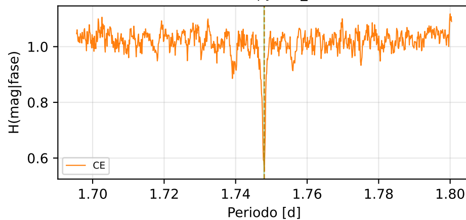
Conditional Entropy (CE_min=0.548)
