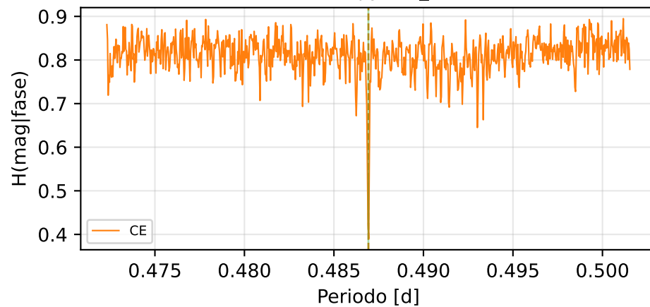
Conditional Entropy (CE_min=0.358)
