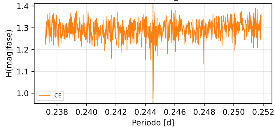
Conditional Entropy (CE_min=0.853)
