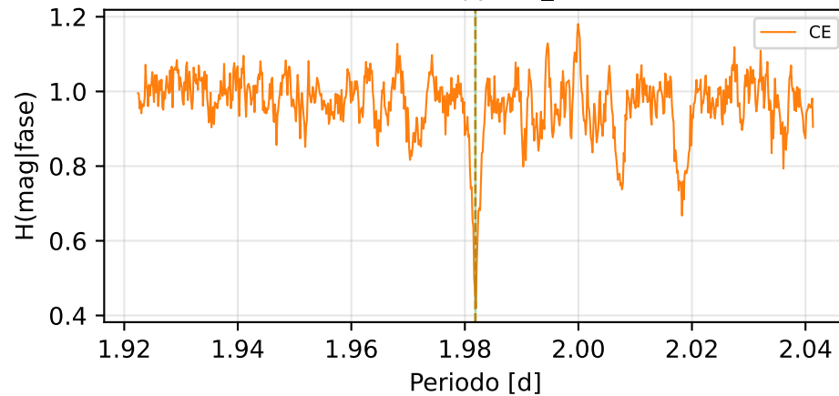
Conditional Entropy (CE_min=0.388)
