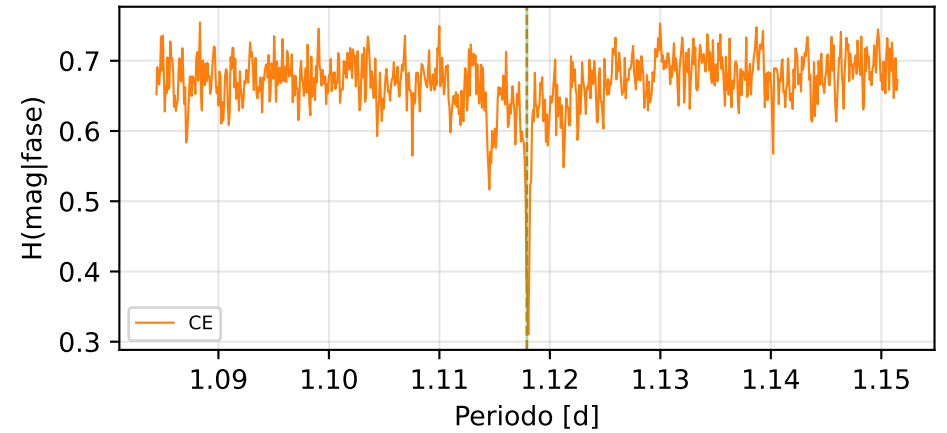
Conditional Entropy (CE_min=0.343)
