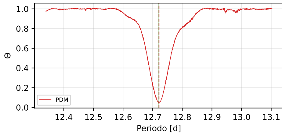
PDM (Theta_min=0.042)
