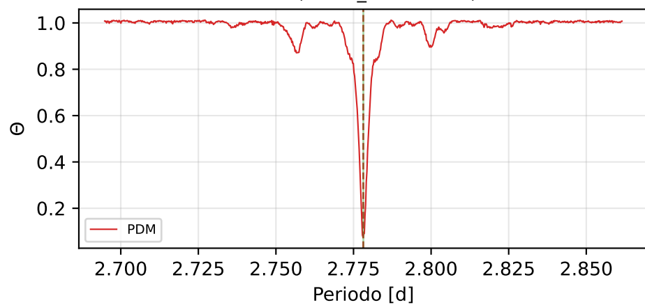
PDM (Theta_min=0.073)
