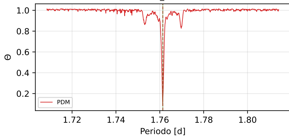
PDM (Theta_min=0.123)
