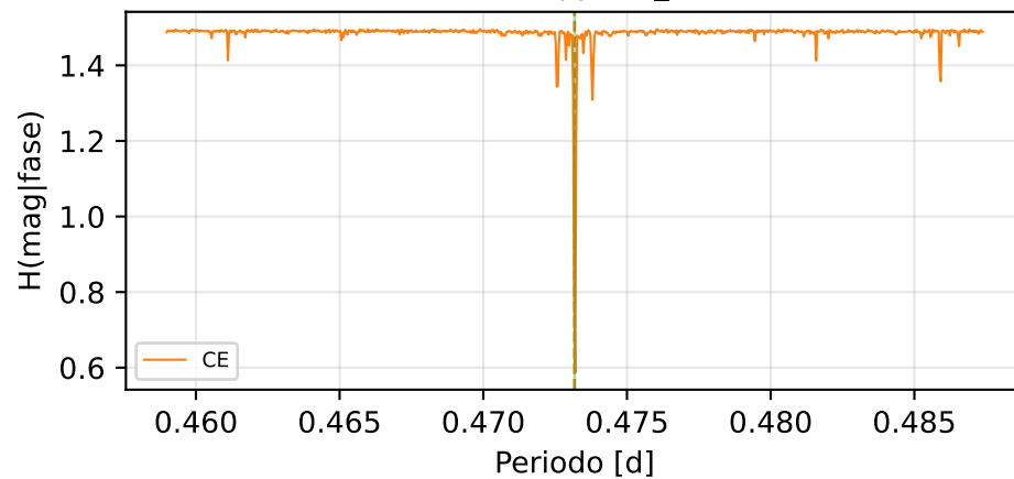
Conditional Entropy (CE_min=0.552)
