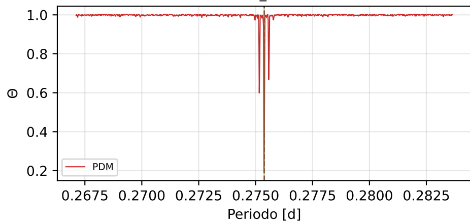
PDM (Theta_min=0.149)
