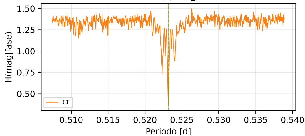
Conditional Entropy (CE_min=0.237)
