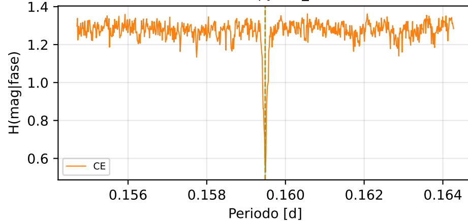
Conditional Entropy (CE_min=0.487)
