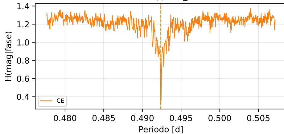
Conditional Entropy (CE_min=0.309)
