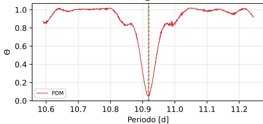
PDM (Theta_min=0.048)
