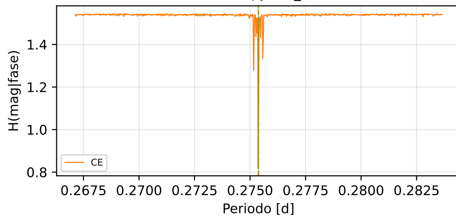
Conditional Entropy (CE_min=0.778)
