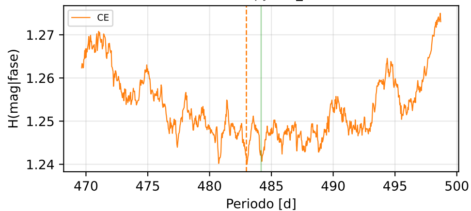
Conditional Entropy (CE_min=1.240)
