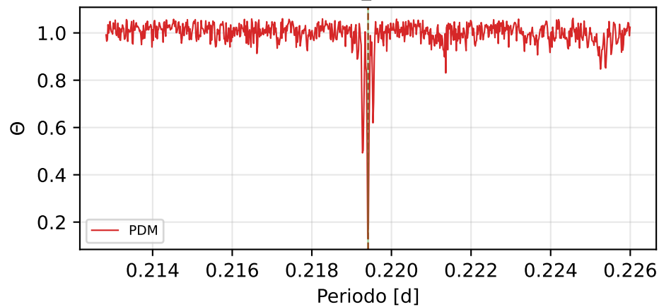
PDM (Theta_min=0.162)
