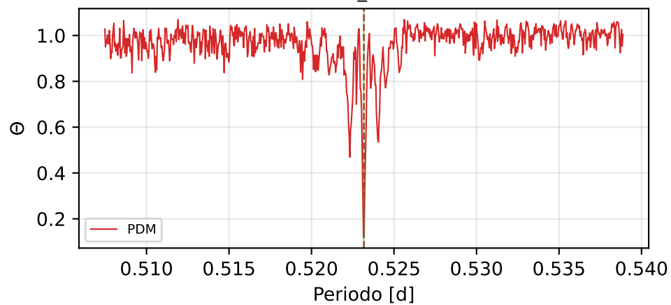
PDM (Theta_min=0.116)
