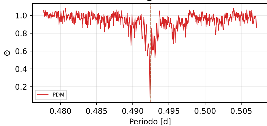
PDM (Theta_min=0.072)
