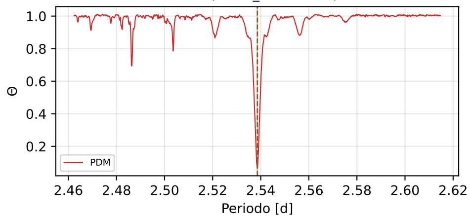
PDM (Theta_min=0.069)
