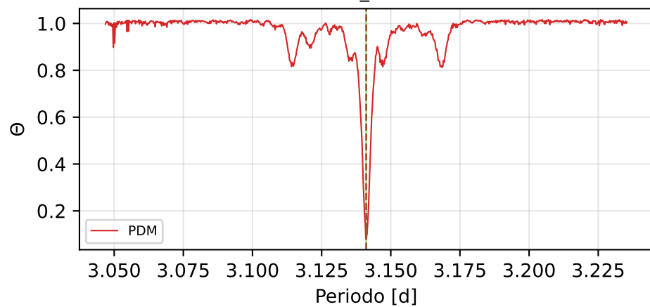
PDM (Theta_min=0.064)
