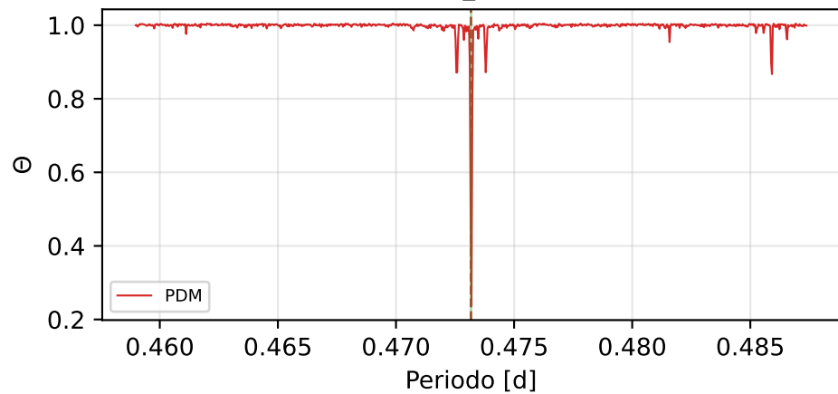
PDM (Theta_min=0.204)
