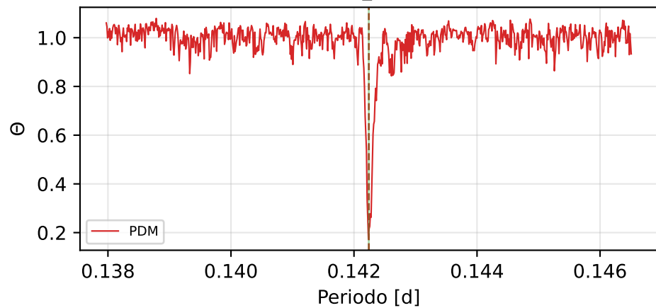
PDM (Theta_min=0.129)
