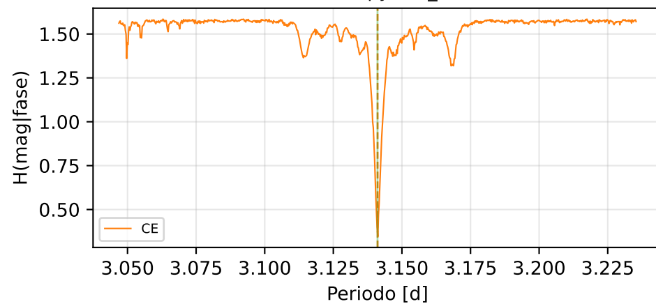
Conditional Entropy (CE_min=0.379)
