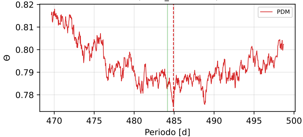
PDM (Theta_min=0.775)
