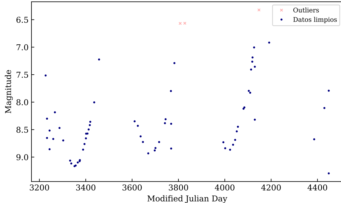
OGLE-LMC-LPV-12184
