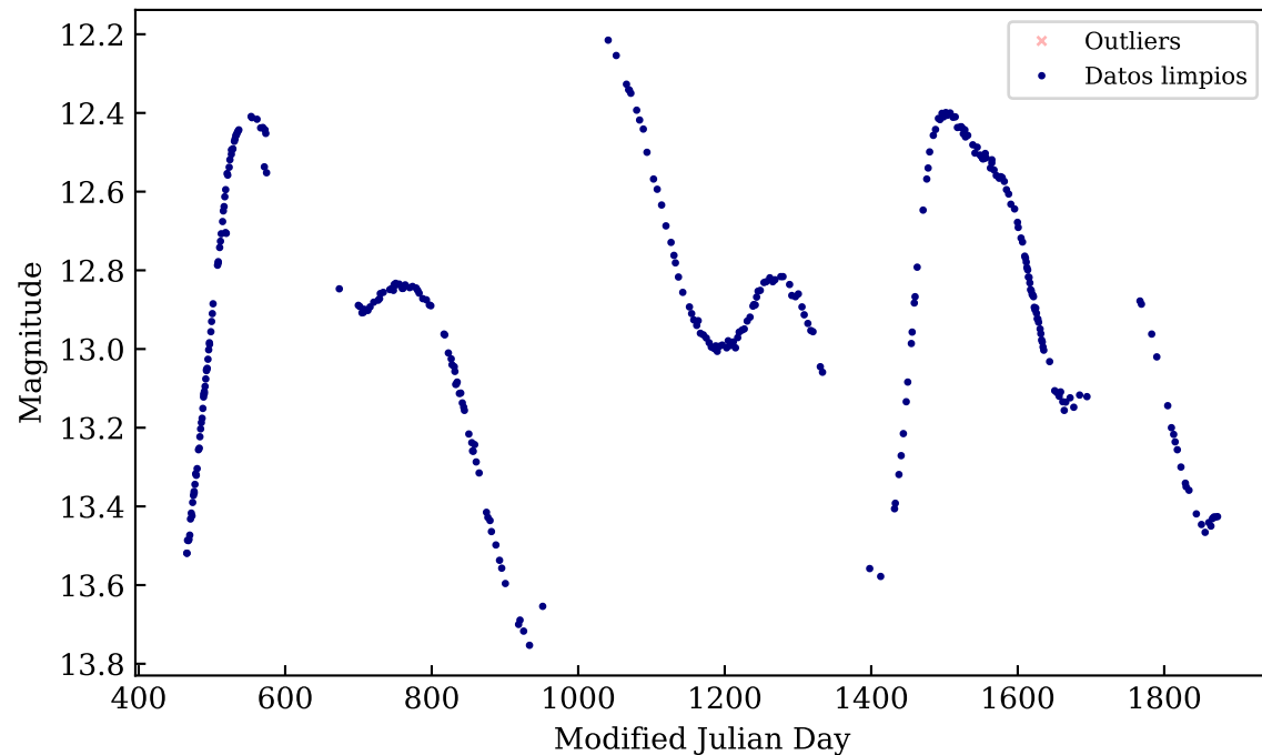
OGLE-LMC-LPV-19063
