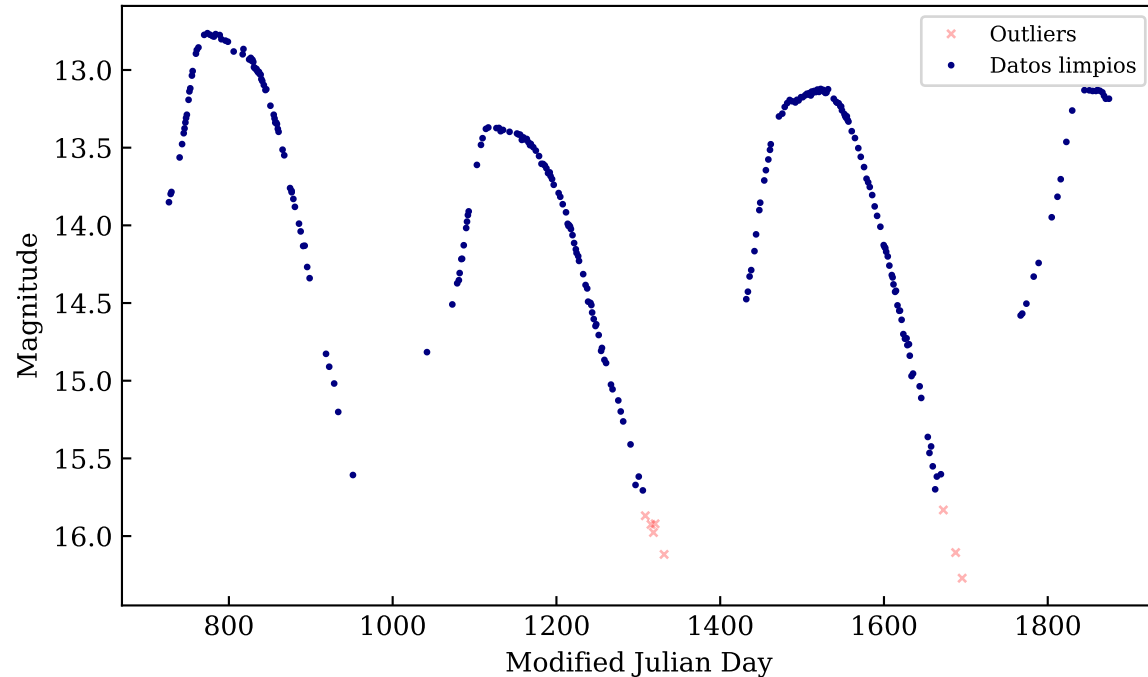
OGLE-LMC-LPV-16796
