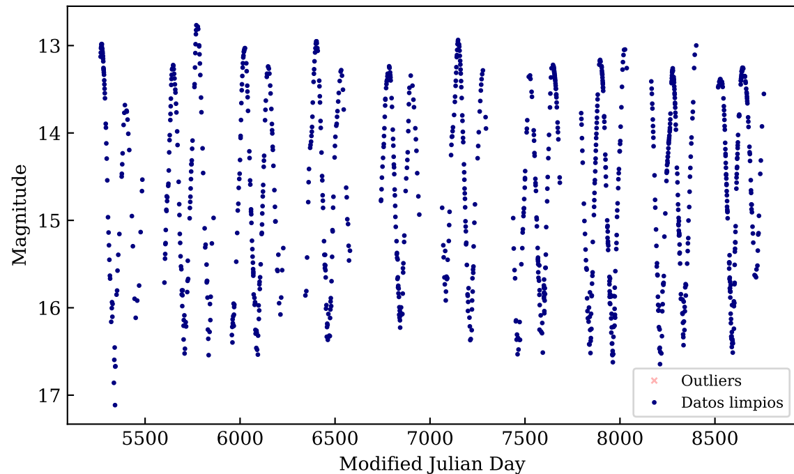
OGLE-BLG-LPV-002715
