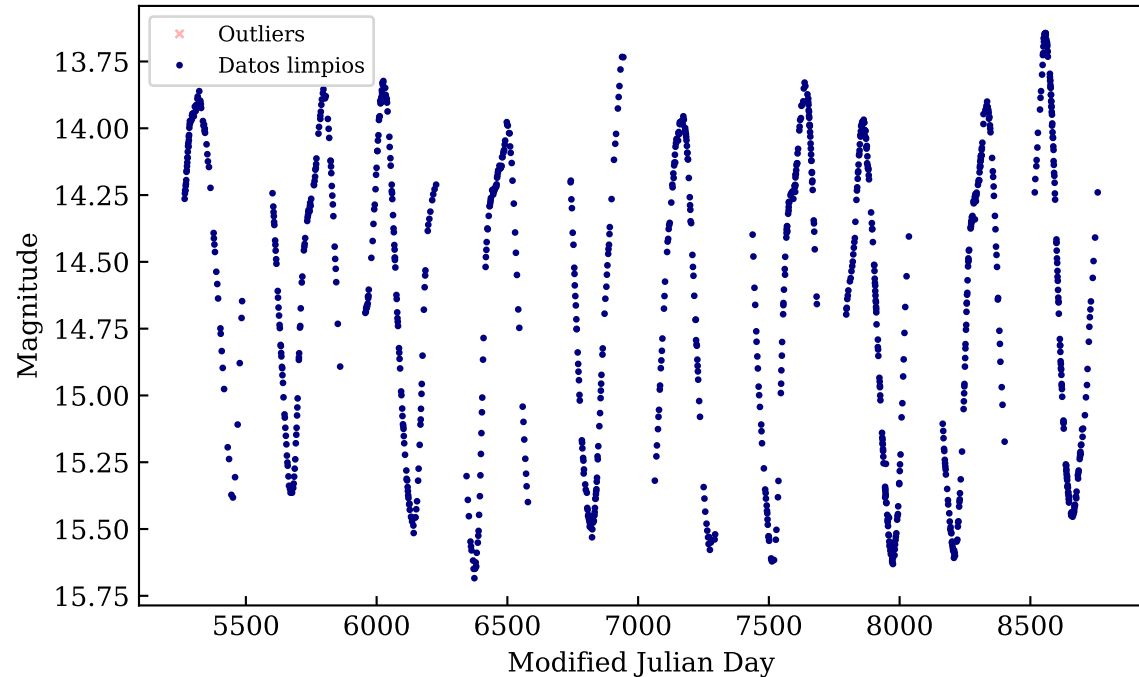
OGLE-BLG-LPV-003971
