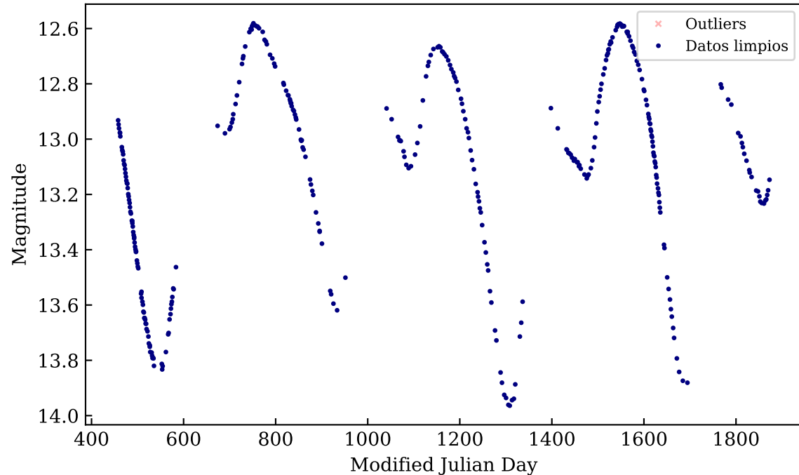
OGLE-LMC-LPV-24564
