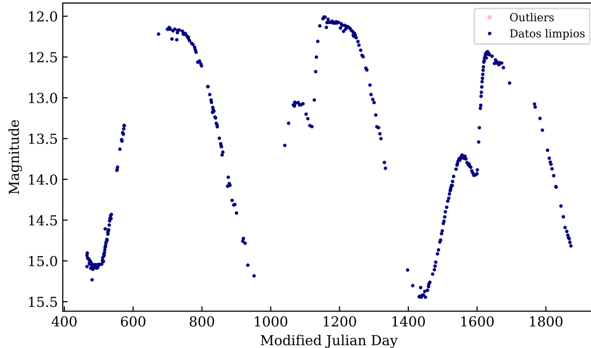
OGLE-LMC-LPV-17853
