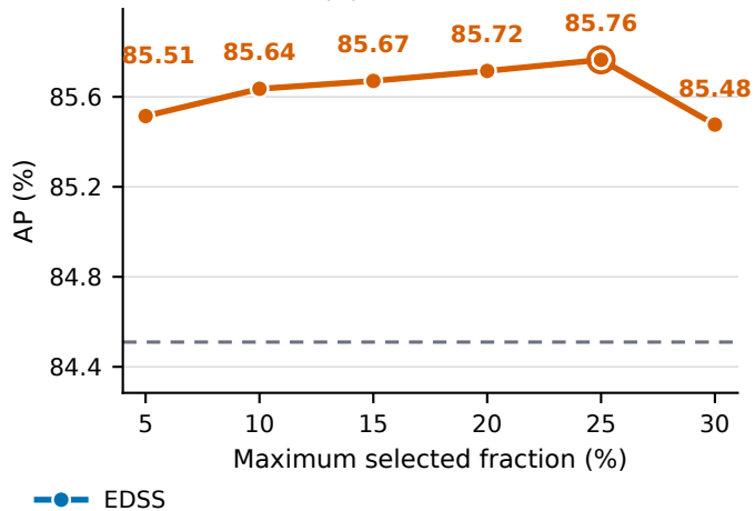
(b) XD-Violence
