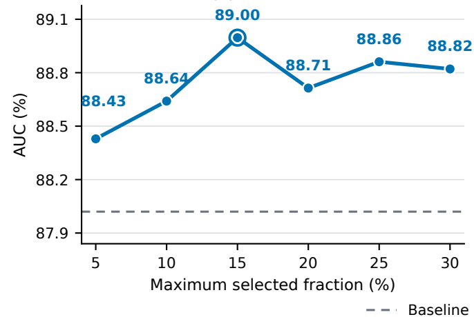
(a) UCF-Crime
