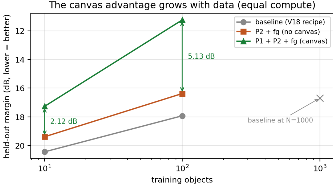
Figure 3: The gap widens with data, which is the argument for a full-dataset run.
