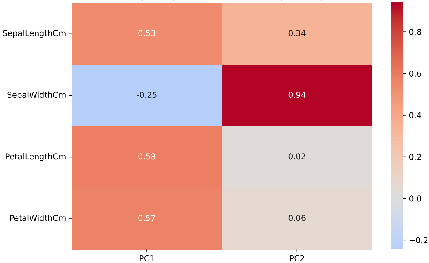
PCA Loadings: Original Features → Principal Components
