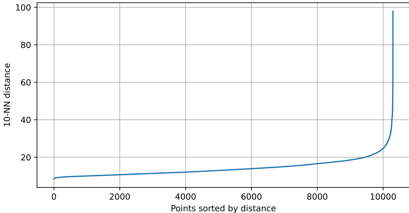
k-distance plot for eps selection
