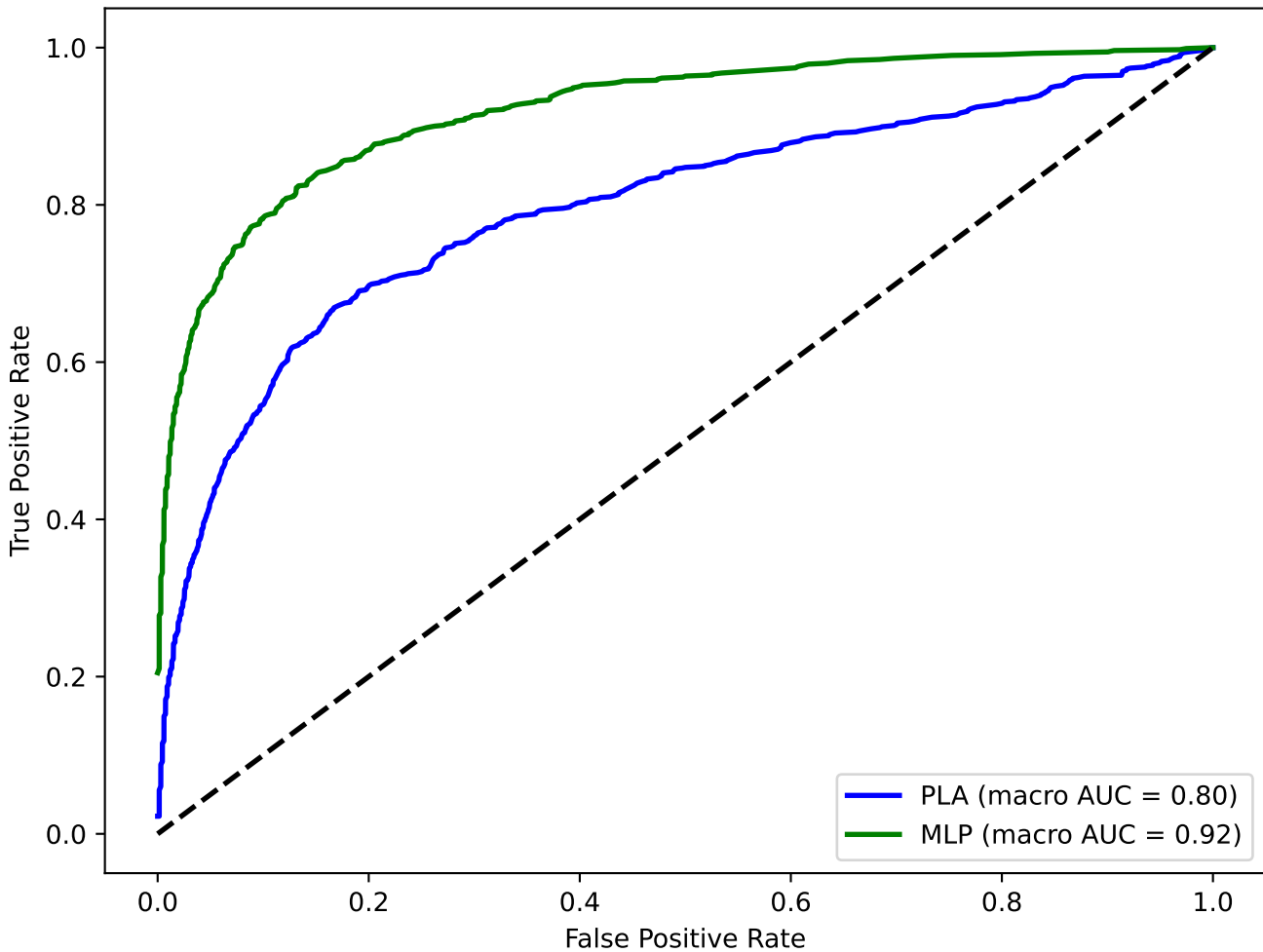
ROC Curves (Macro Average)
