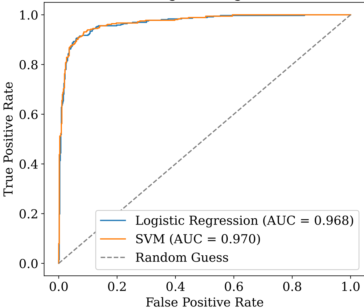
ROC Curve - Logistic Regression vs SVM
