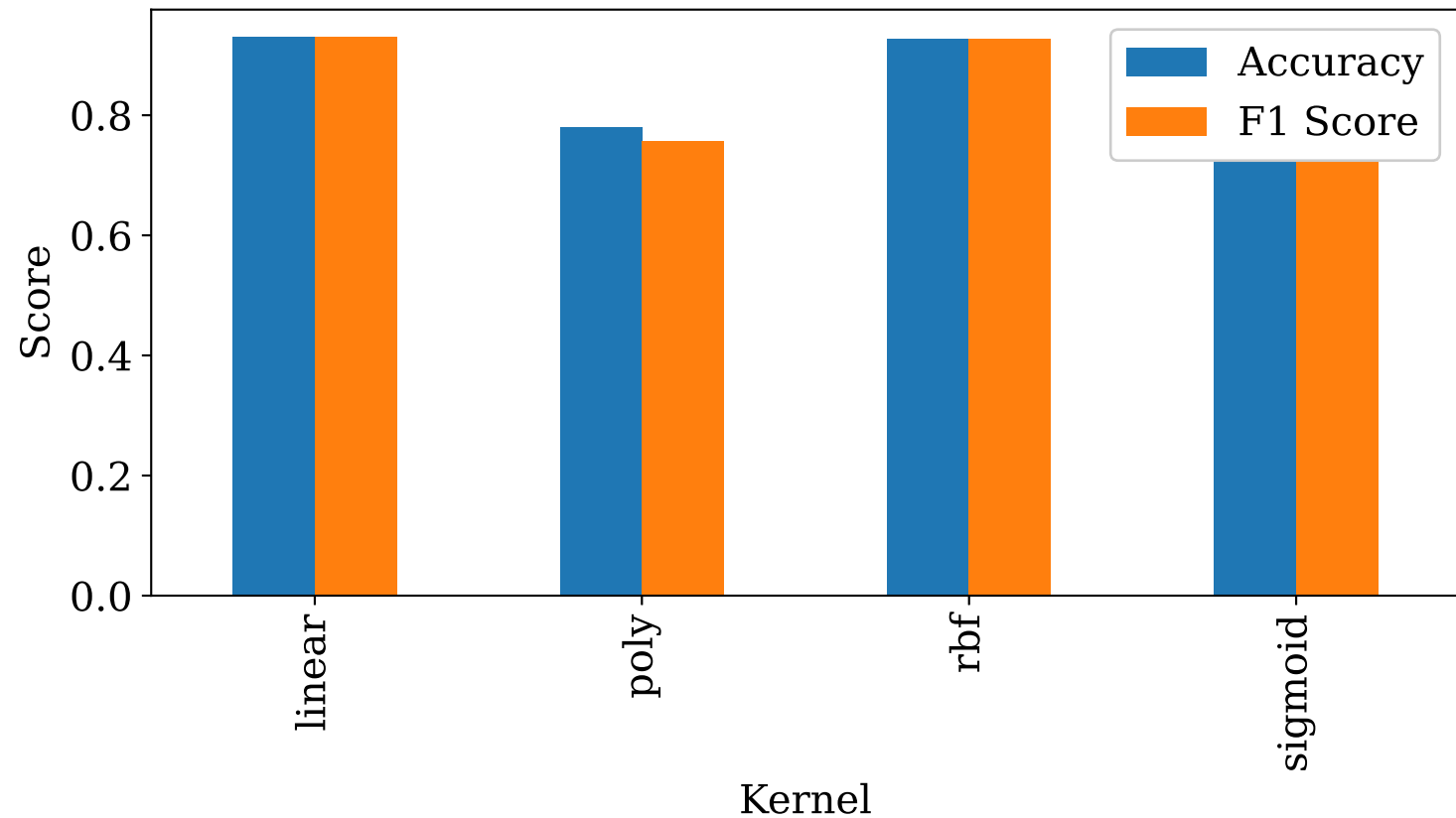
SVM Kernel-wise Performance
