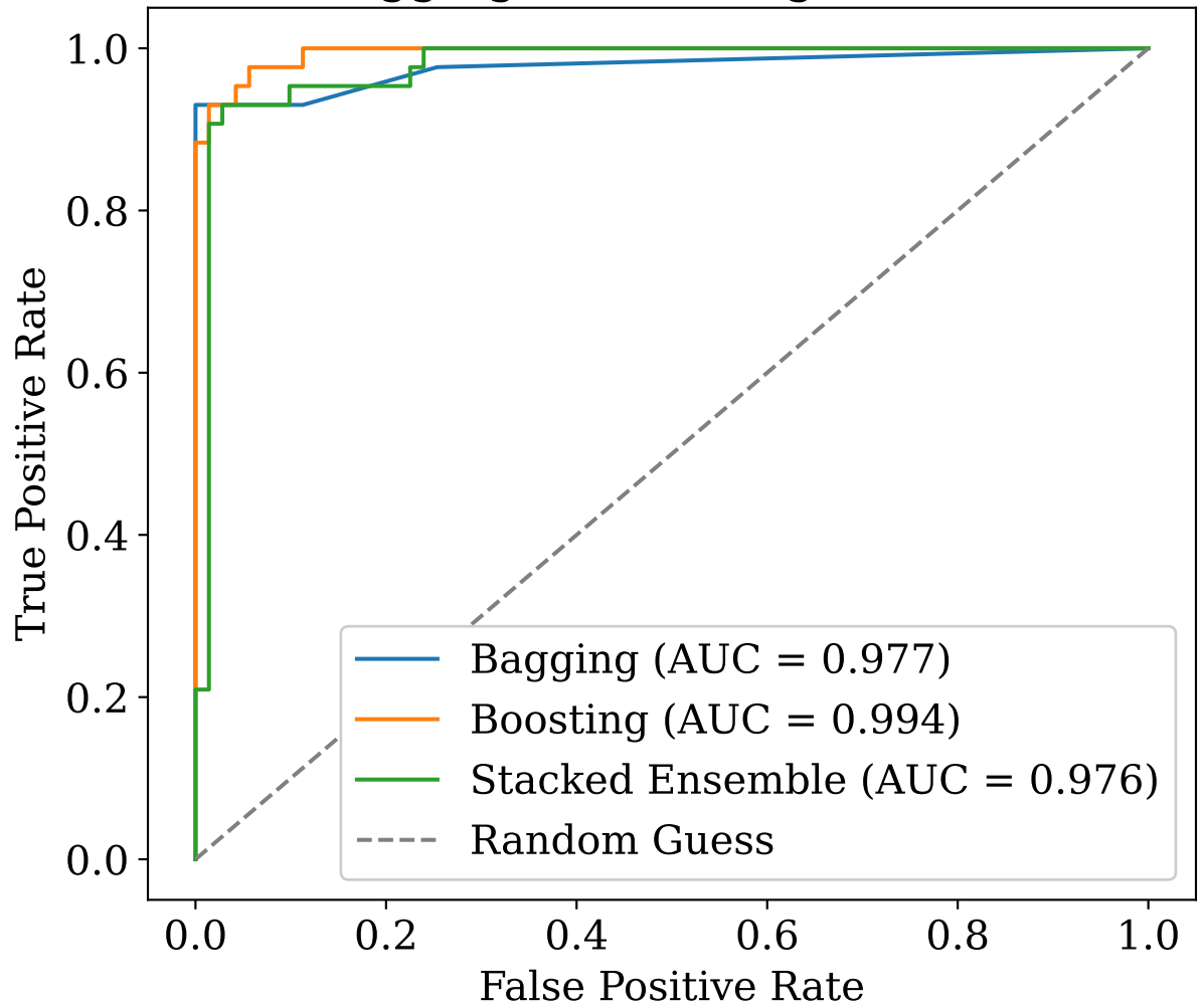
ROC Curve - Bagging vs Boosting vs Stacked Ensemble
