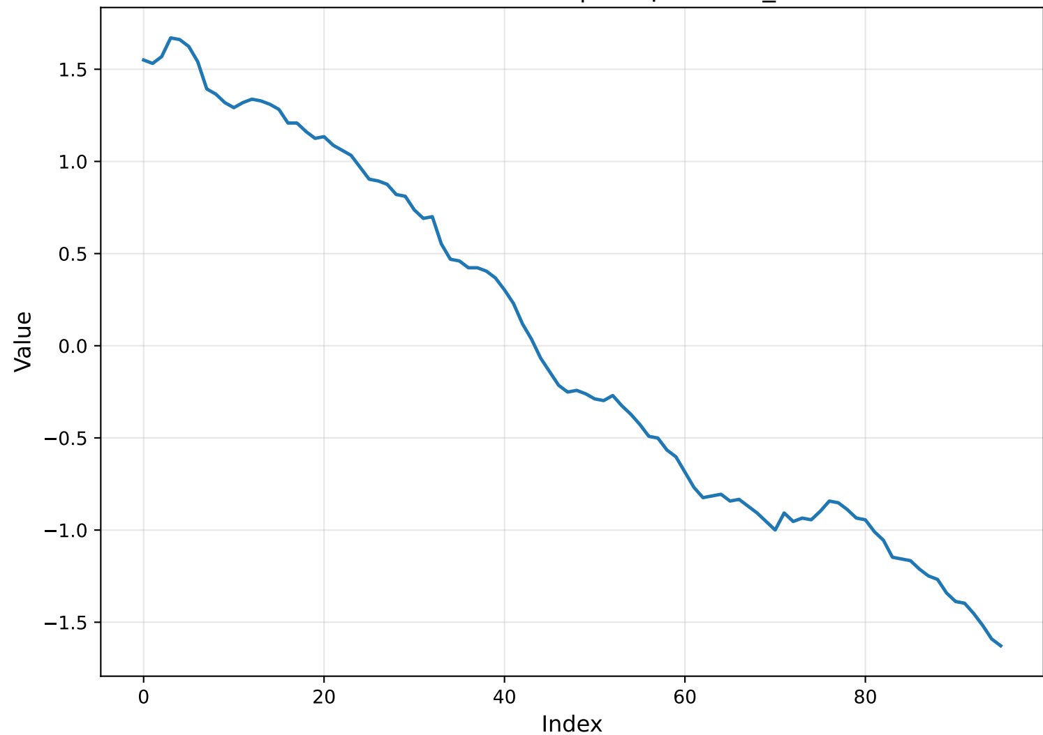
after noDiffusion | sample0 ch0_1
