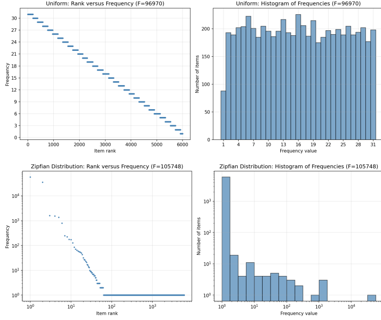
Figure 1: The rank-frequency and histogram plots for the two synthetic stream generation settings.
