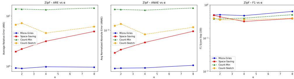
Figure 4: Effect of \alpha on ARE, ANAE, and F_1 score for the Zipf distribution (fixed memory, F = 50,000 ).
