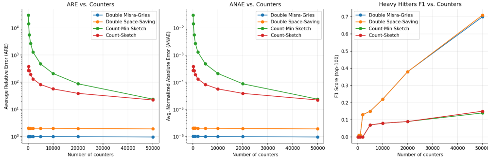
Figure 7: Effect of counter budget on accuracy for the idle-timeout stream ( \alpha = 1.0015 , \|\mathbf{f}\|_1 = 998,717 ). Even with near-absence of deletions, counter-based algorithms maintain their advantage; sketches suffer from large additive errors.
