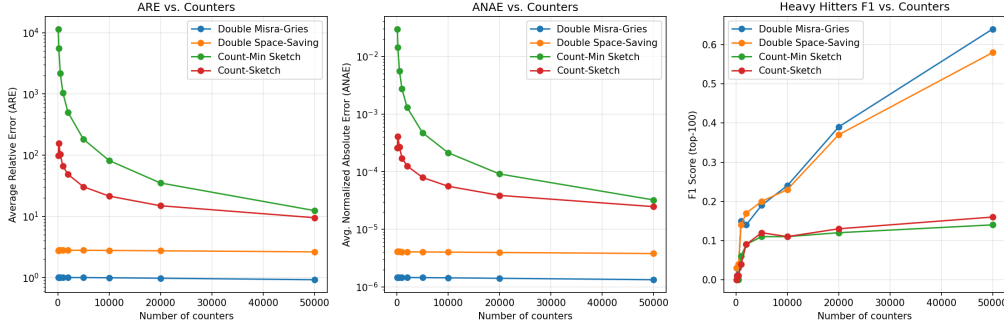
Figure 6: Effect of counter budget on accuracy for the sliding-window stream ( \alpha = 2.5993 , \|\mathbf{f}\|_1 = 384,724 ). Left: ARE, center: ANAE, right: F_1 score. All metrics improve with more counters; counter-based algorithms significantly outperform sketches.
