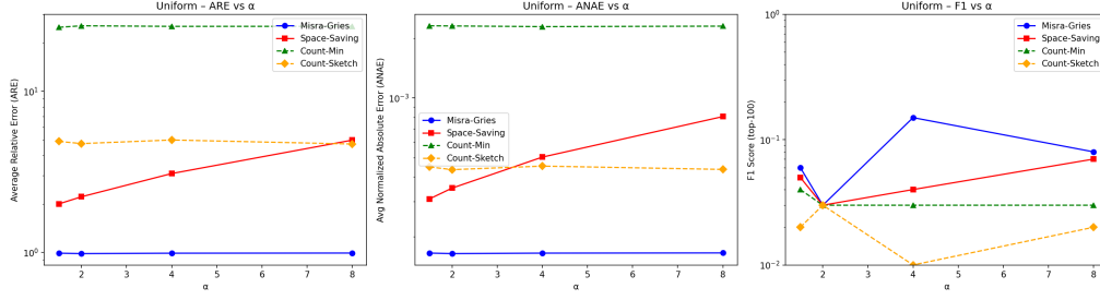
Figure 5: Effect of \alpha on ARE, ANAE, and F_1 score for the Uniform distribution (fixed memory, F = 50,000 ).
