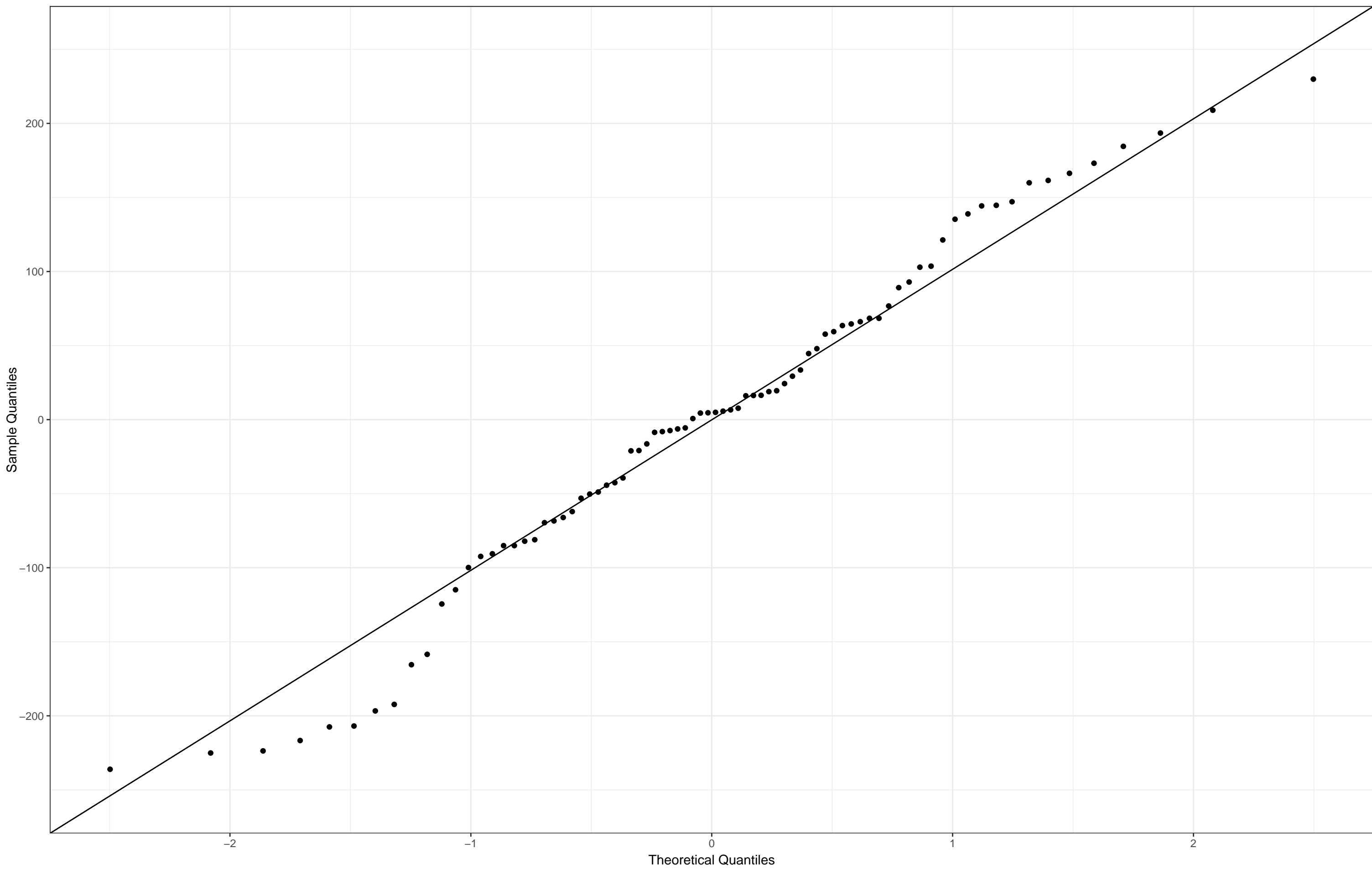
QQ-Plot of Residuals
