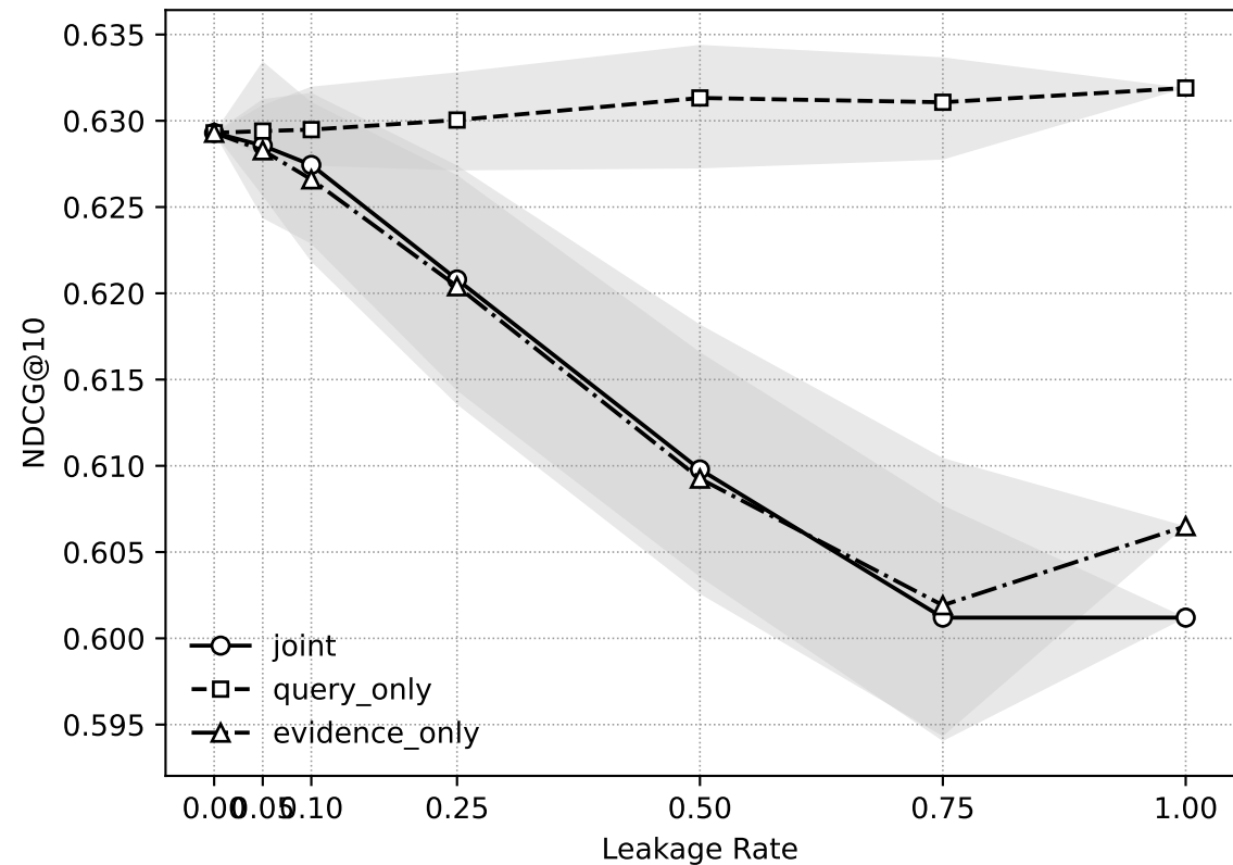
NDCG@10 vs Leakage Rate
