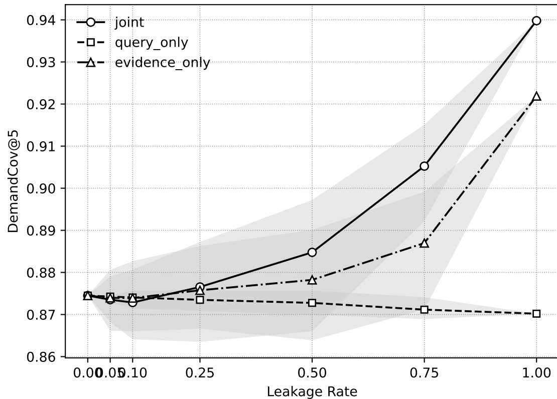
DemandCov@5 vs Leakage Rate
