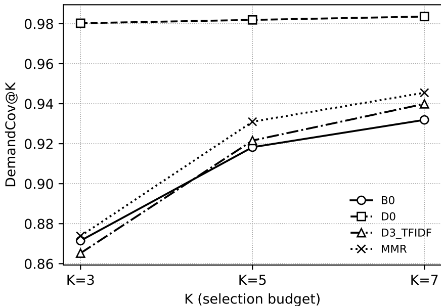
DemandCov@K by K — internal_blind
