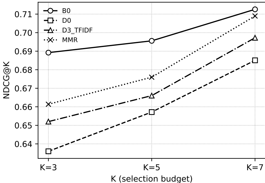
NDCG@K by K — cmedqa2_external
