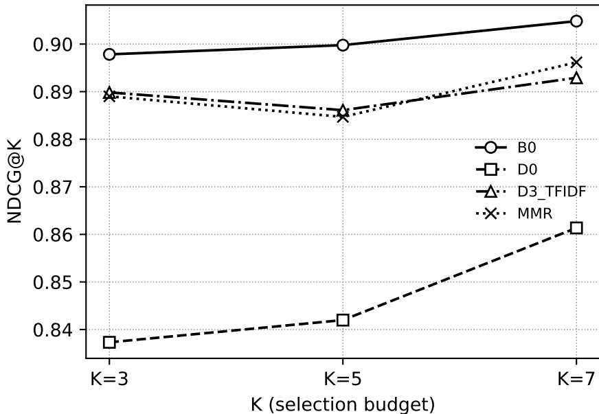
NDCG@K by K — formal_train
