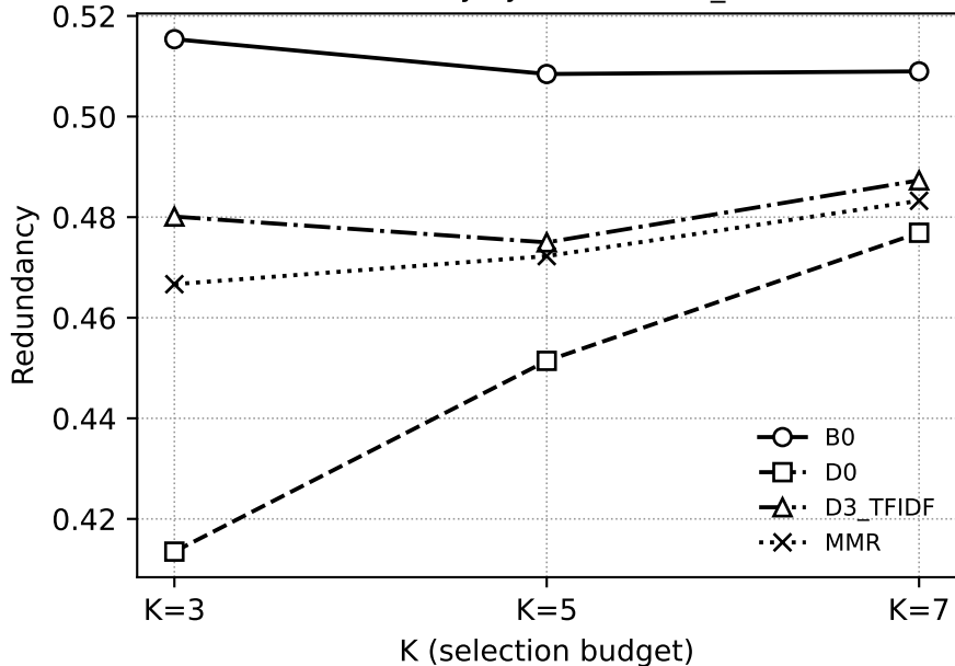
Redundancy by K — internal_blind
