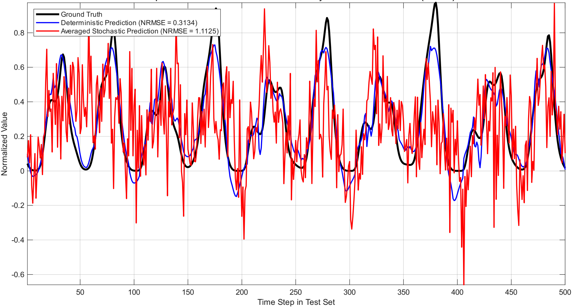
Comparison of Model Predictions on Mackey-Glass Cubed Test Set (Iter 91)
