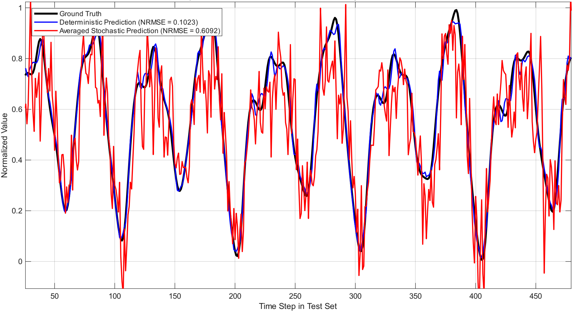
Comparison of Model Predictions on Mackey-Glass Test Set
