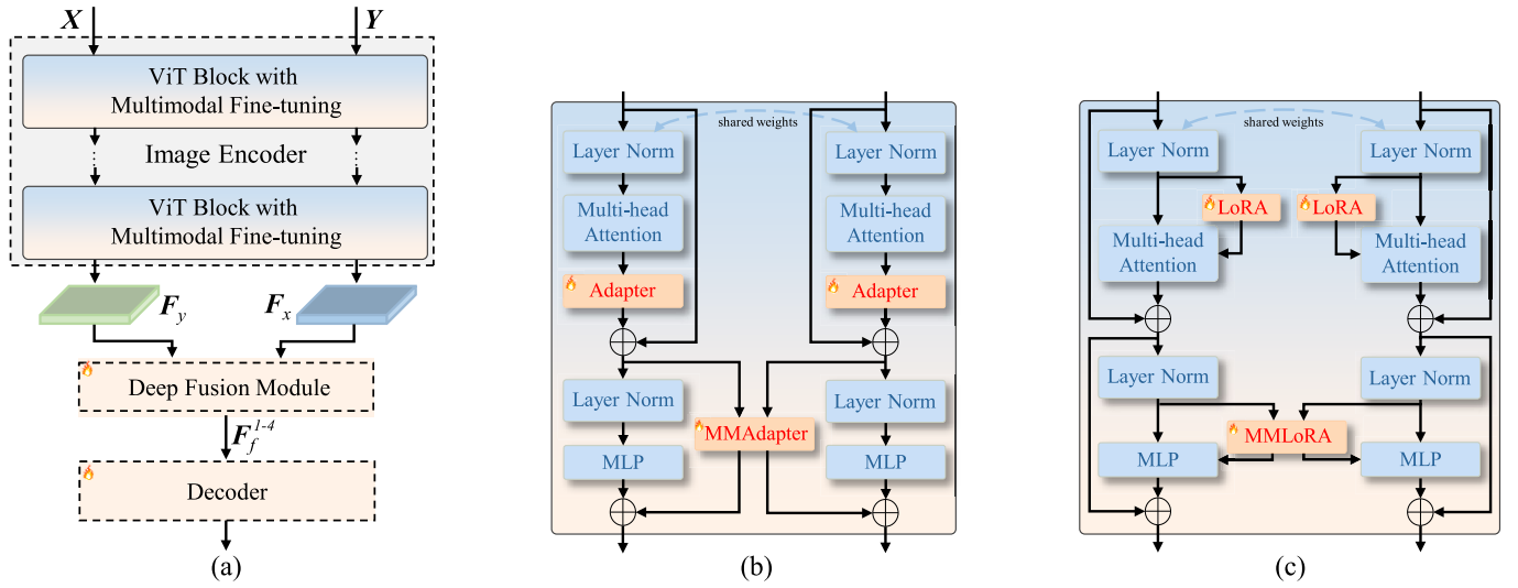
Fig. 5. (a) Overview of the proposed MFNet consisting of an SAM's image encoder with multimodal fine-tuning, a DFM, and a general decoder. The structure of (b) ViT block with MMAdapter and (c) ViT block with MMLoRA. These constitute the two distinct architectures of MFNet.
