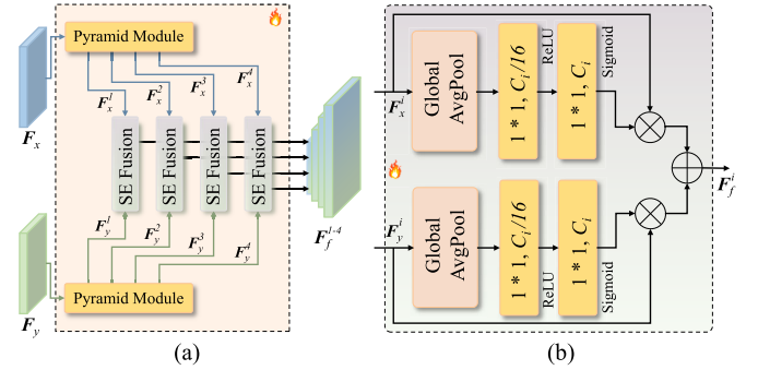
Fig. 6. (a) Schematic of the DFM. There are two pyramid modules that expand multimodal features for multiscale features before they are fused by four SE fusion modules. (b) Schematic of the SE fusion module [33]. Notably, we just employ the existing simple fusion module and do not design this structure specifically, which proves that our primary gains are derived from the multimodal fine-tuning strategy based on the vision foundation model.
