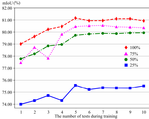
Fig. 12. Relationship between training data volume and model performance during the training stage. As the model is unable to generate predictions in the absence of training data, we designed and carried out experiments with three levels of training data availability: 25%, 50%, and 75%, in addition to using the complete training set (100%).
