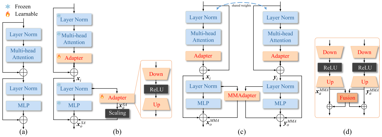
Fig. 3. (a) ViT block without Adapter in SAM's image encoder, (b) ViT block equipped with standard Adapter [37], (c) ViT block endowed with the proposed MMAAdapter, and (d) detailed structure of the MMAAdapter. The Adapter facilitates the efficient utilization of general knowledge in specific tasks. Compared to the standard Adapter, MMAAdapter is characterized by two branches of shared weights for multimodal feature extraction. The standard Adapter and the proposed MMAAdapter are used to fine-tune and fuse features, respectively.
