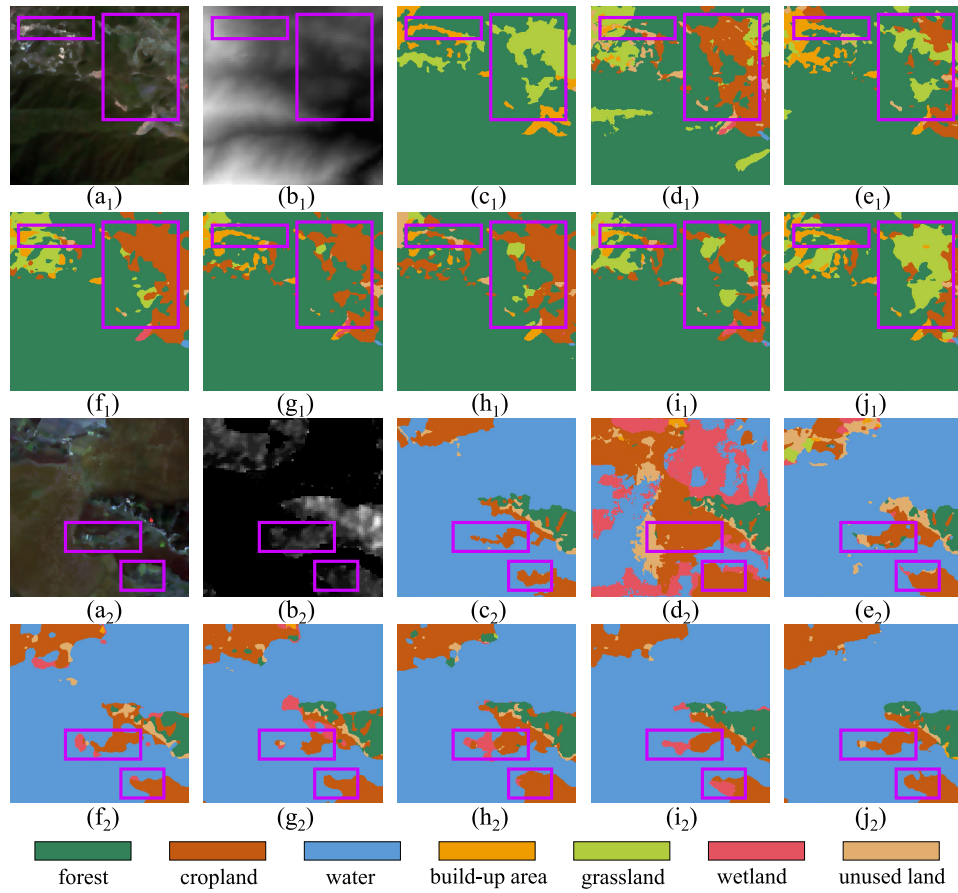
Fig. 10. Visualized comparisons on the MMHunan test set with the size of 256 \times 256 and 1024 \times 1024 . (a) IRRG images, (b) DSM, (c) ground truth, (d) CMFNet, (e) FTransUNet, (f) MFTransNet, (g) CMGFNet, (h) FTransDeepLab, (i) MultiSenseSeg, and (j) proposed MFNet. To highlight the differences, some purple boxes are added to all subfigures. Subscripts (=1, 2) represent the serial number of the samples displayed.
