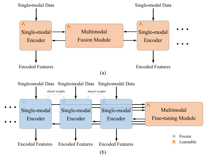
Fig. 2. (a) Current multimodal fusion methods and (b) proposed unified multimodal fine-tuning framework. In our method, single-modal encoders are used to learn general knowledge and frozen, enabling multimodal tasks to benefit from the vision foundational model.
