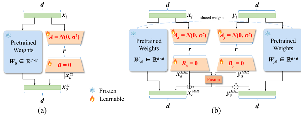
Fig. 4. (a) Detailed structure of standard LoRA [27] and (b) proposed MMLoRA. It is observed that MMLoRA adopts the design principles of MMAdapter, which not only reduces the module's complexity but also highlights the versatility of this strategy.
