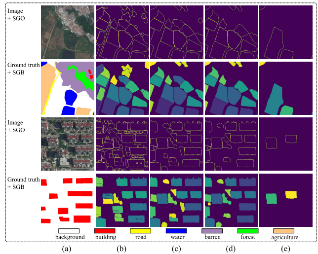
Fig. 9. (a) Image and corresponding ground truth on the LoveDA Urban dataset. Visual examples of SGO and SGB when “pred_iou_thresh” is set to (b) 0.50, (c) 0.95, (d) 0.96, and (e) 0.99.
