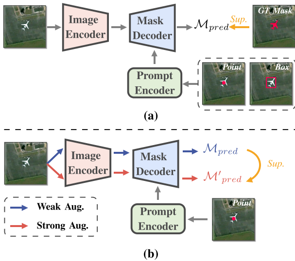
Fig. 1. (a) Training pipeline of vanilla SAM. (b) Training pipeline of self-training based PointSAM. Sup. means supervise.
