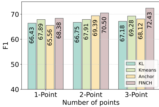
Fig. 6. Comparison of the different feature clustering and alignment methods on the HRSID-inshore dataset.
