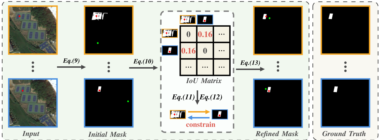
Fig. 4. Process of NPC. The positive and negative prompts are represented by red points ( \bullet ) and green points ( \circ ), respectively. Different prompts input into SAM generate different initial masks. To refine these masks, an IoU matrix is calculated for each instance pair. Matrix values greater than 0 indicate that the two objects can act as negative constraints for each other. By using the positive prompt of one object as the new negative prompt for another and inputting it into SAM again, a refined mask is generated. It is worth noting that GT here refers to the mask specified by the prompt for a specific instance, not the mask for all instances.
