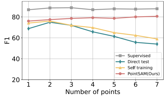
Fig. 7. Impact of the number of points on different methods on the NWPU VHR-10 dataset.
