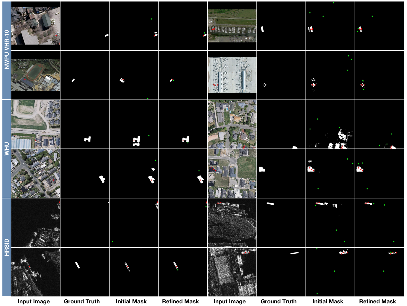
Fig. 8. Visualization of NPC results during training. Positive prompts are marked with red points (●), while negative prompts are marked with green points (●). The refined mask is obtained by applying NPC to the initial mask. This calibration effectively guides the negative prompts to more precise regions, resulting in improved mask predictions.
