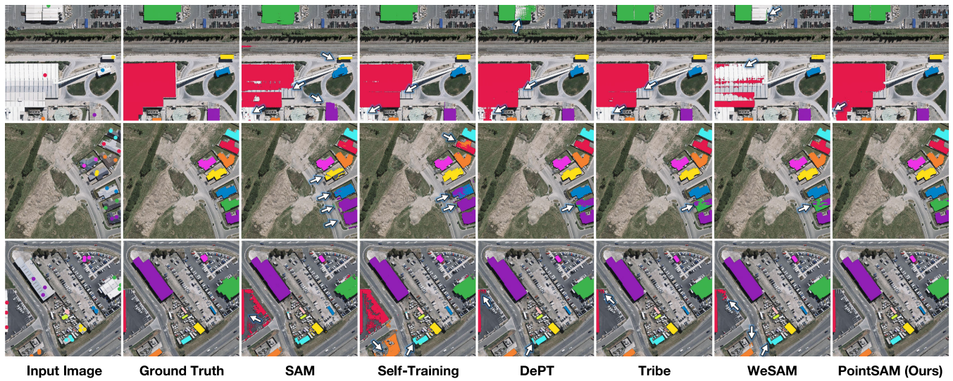
Fig. 10. Comparative results of different methods on the WHU dataset. Rows 1–3 present the results under one, two, and three prompts, respectively. White arrows in the images are used to highlight the detail.
