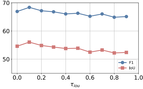
Fig. 5. Impact of different thresholds of IoU on the HRSID-inshore dataset with one point.
