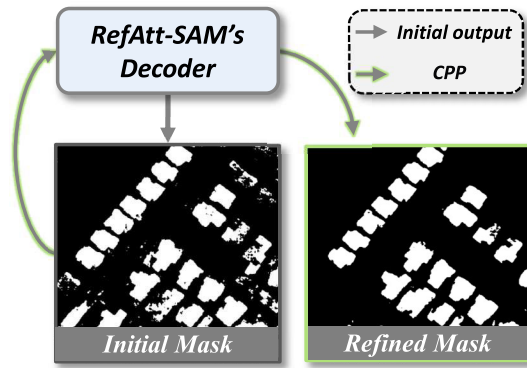
Fig. 4. Pipeline of CPP.
