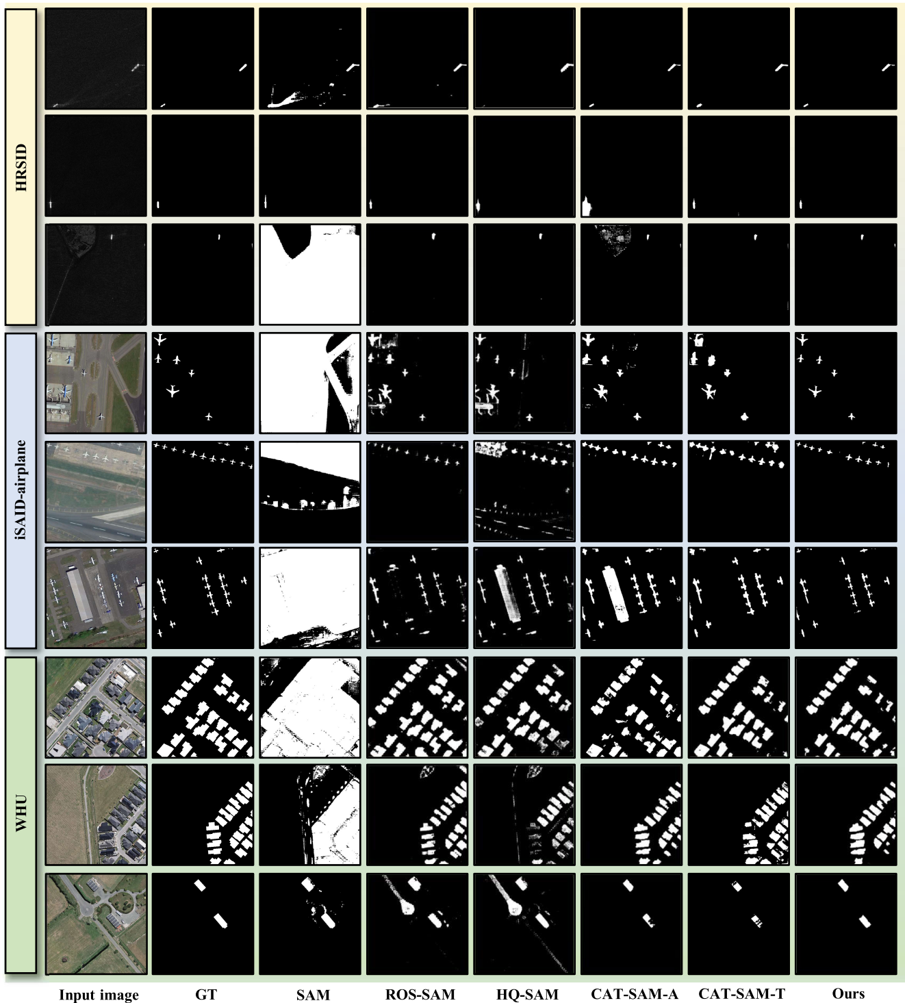
Fig. 5. Qualitative comparison of different methods on the HRSID, iSAID, and WHU datasets.
