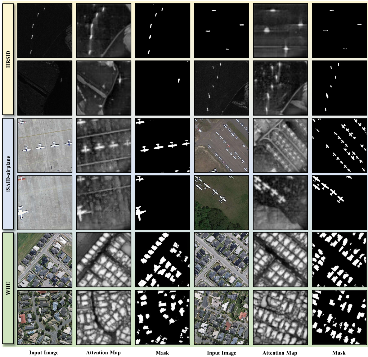
Fig. 6. Visualizations of FAM.
