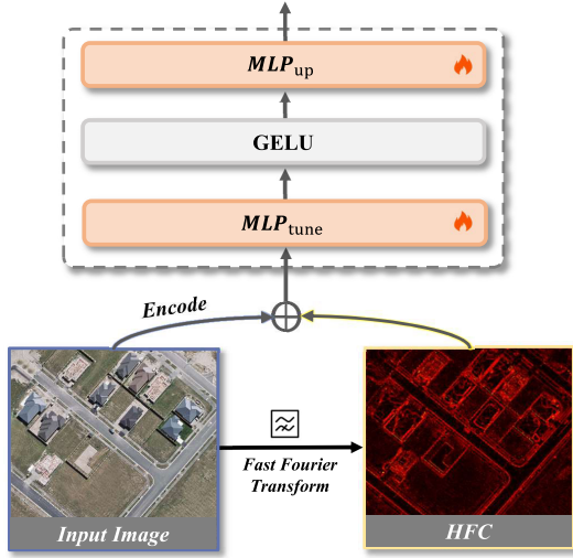
Fig. 3. Structure of the HF-Adapter, where the HFCs capture the edge information of the image and are highlighted with red lines.
