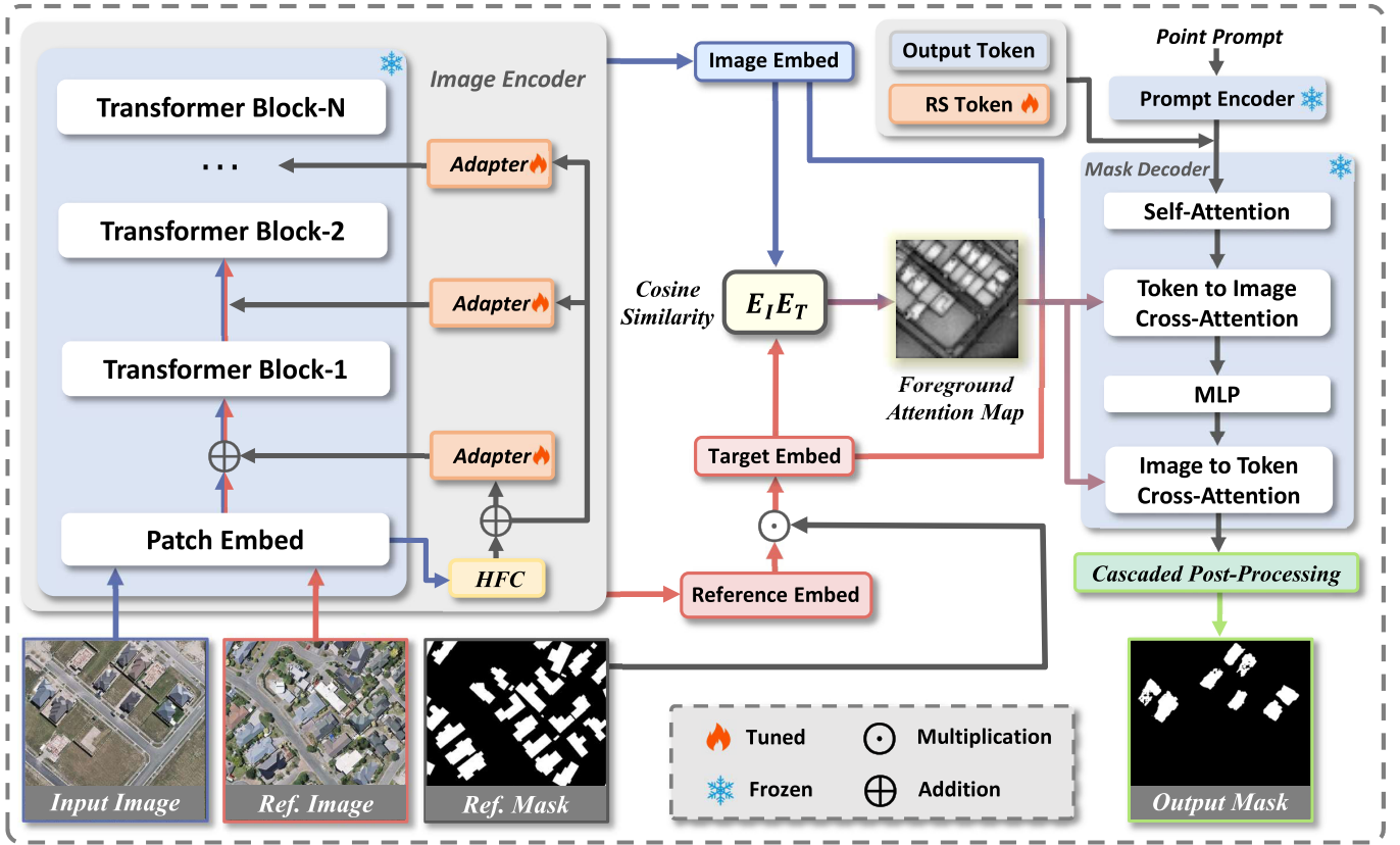
Fig. 2. Overall structure of RefAtt-SAM. During the training stage, RefAtt-SAM keeps the original image encoder and mask decoder of SAM frozen and only adjusts the inserted Adapter and RS-Token. During the inference stage, the model obtains the target features from a reference image with a mask. Subsequently, it calculates the cosine similarity between these features and those of the test image to generate an FAM. Finally, this map is fed into the mask decoder for cross-attention, enabling the network to focus more on the foreground and thereby produce high-quality masks.
