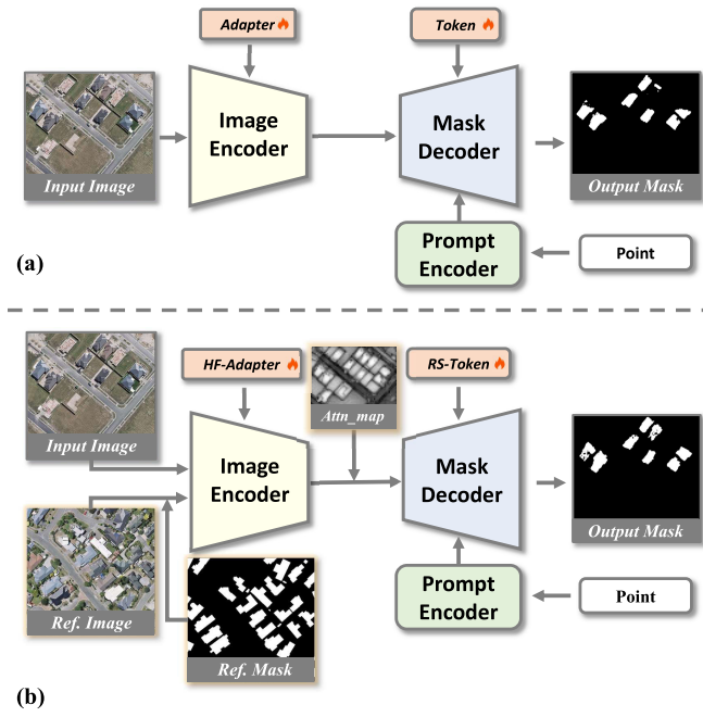
Fig. 1. (a) CAT-SAM. (b) Proposed RefAtt-SAM. Attn_map denotes the FAM. Ref. denotes reference.
