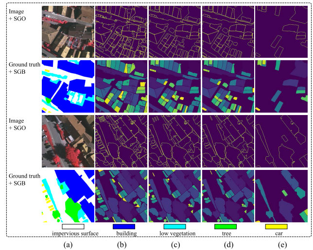
Fig. 8. (a) Image and corresponding ground truth on the ISPRS Vaihingen dataset. Visual examples of SGO and SGB when “pred_iou_thresh” is set to (b) 0.50, (c) 0.95, (d) 0.96, and (e) 0.99.
