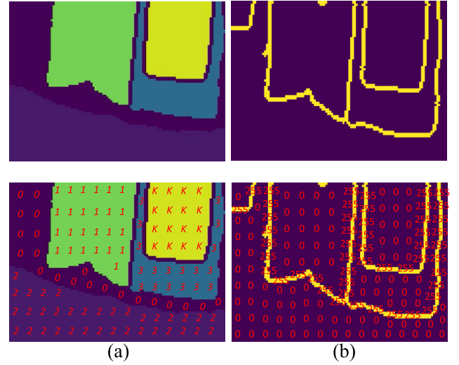
Fig. 4. (a) SGO and its diagram with pixel values where the pixels inside the same object have the same value, and the maximum index is the threshold K . (b) SGB and its diagram with pixel values. The boundary pixels are set to 255, while others are set to 0.
