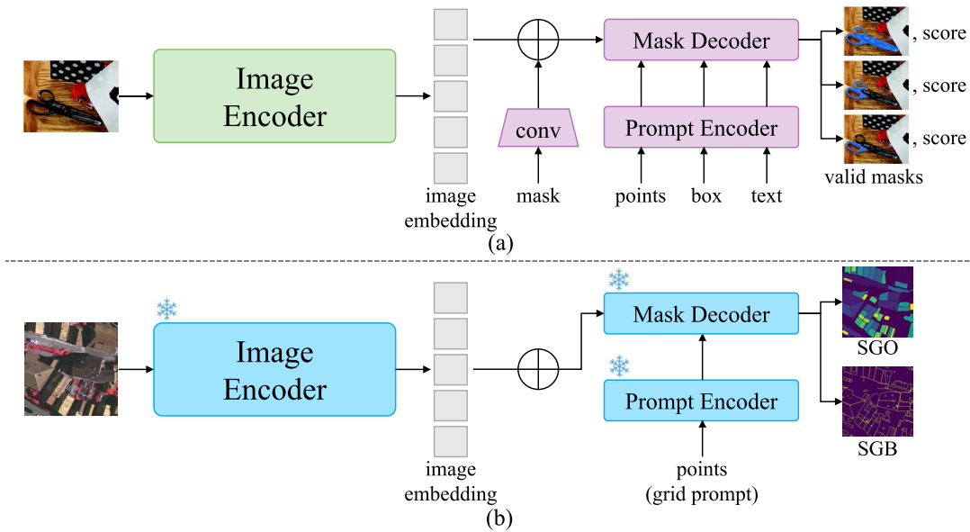
Fig. 2. Comparison of frameworks between SAM and the proposed approach. (a) Schematic of the SAM framework [32]. (b) Schematic of the proposed SAM-based pre-processing approach. All parameters of SAM are frozen, and SGO and SGB are generated with grid prompt. It is the only mode that automatically segment the entire image by creating multiple point prompts using a regular grid.
