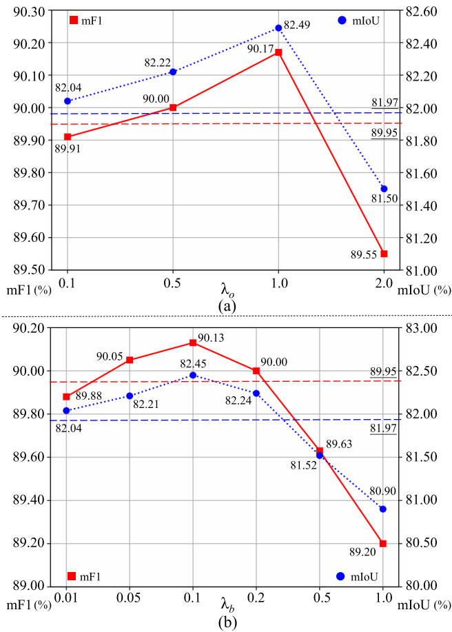
Fig. 10. Sensitivity analysis of (a) \lambda_o and (b) \lambda_b on the ISPRS Vaihingen dataset. The performance of the baseline is depicted using dashed lines to highlight the variation of performance.
