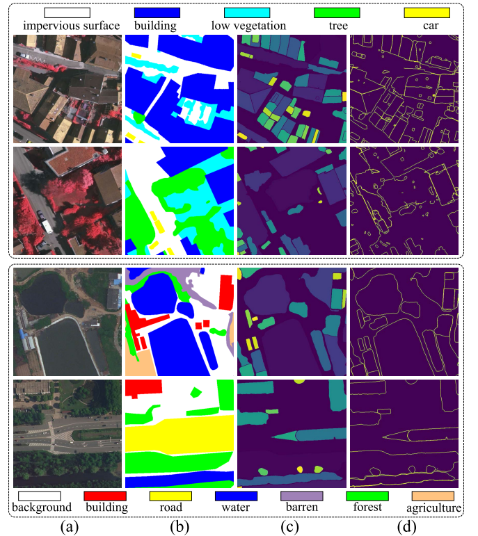
Fig. 1. Visual examples. (a) Images. (b) Ground truth. (c) SGO. (d) SGB. The first two rows show samples of size 512 \times 512 from ISPRS Vaihingen. The last two rows show samples of size 512 \times 512 from LoveDA Urban. It can be observed that SGO and SGB provide a wealth of detailed information about ground objects from both object and boundary perspectives.
