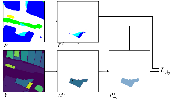
Fig. 5. Flowchart for computing object consistency loss.
