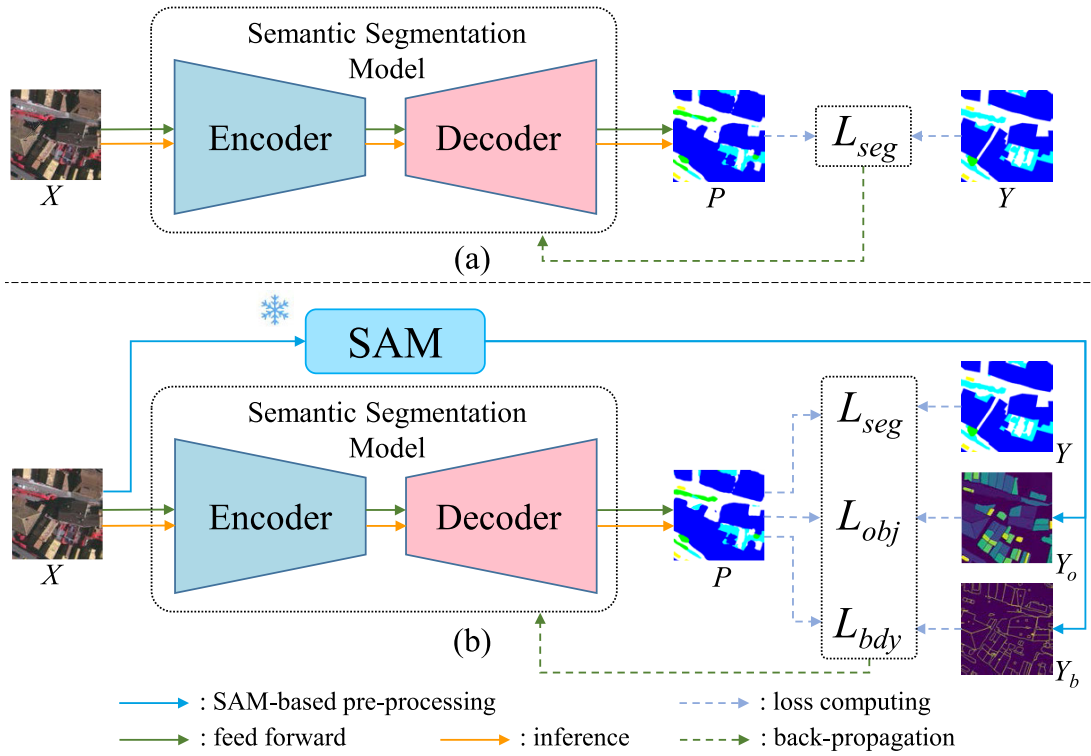
Fig. 3. (a) Schematic of the general semantic segmentation model. (b) Schematic of the proposed method. In the proposed method, the image X is fed into the semantic segmentation model that generates the segmentation output P before the segmentation loss L_{seg} is computed by segmentation output and ground truth Y , which is used for backpropagation to update the model. Meanwhile, two additional loss functions L_{obj} and L_{bdy} are computed by SGO Y_o and SGB Y_b , which will also be used for model optimization together with L_{seg} .
