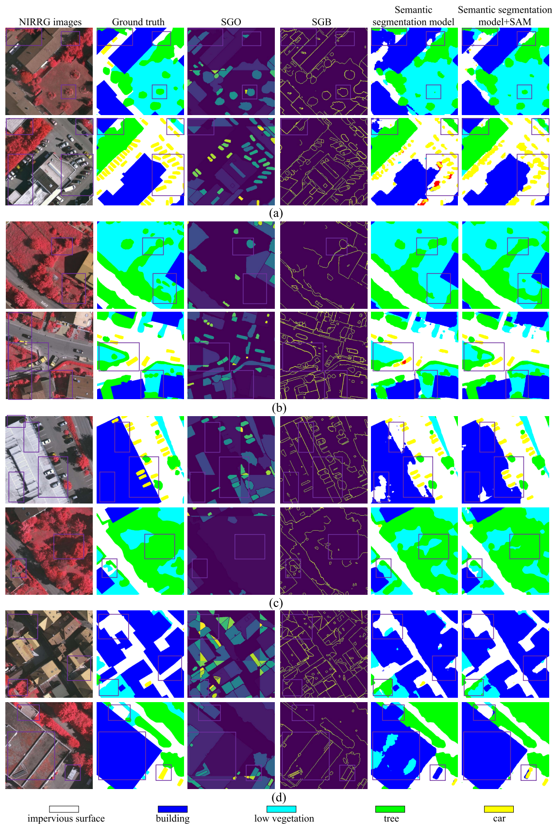
Fig. 6. Qualitative performance comparisons on the ISPRS Vaihingen with the size of 512 \times 512 . (a) ABCNet. (b) CMTFNet. (c) UNetformer. (d) FTUNetformer. We showcase two samples for each model. Some purple boxes are added to highlight the differences.
