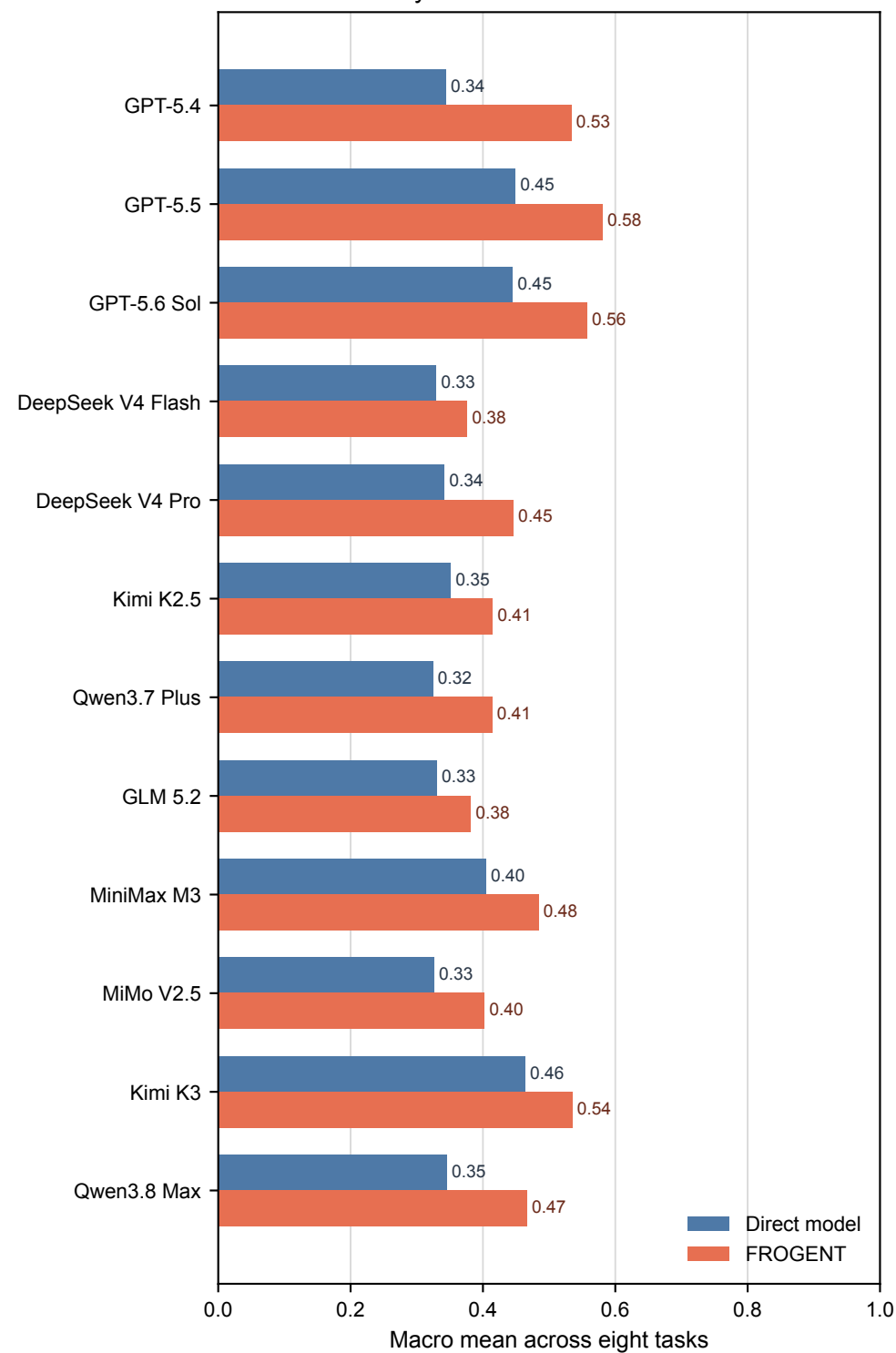
System-level model effect
