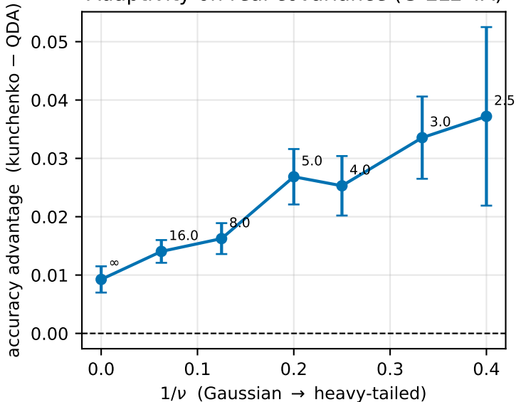
Adaptivity on real covariance (G-ELL-4A)
