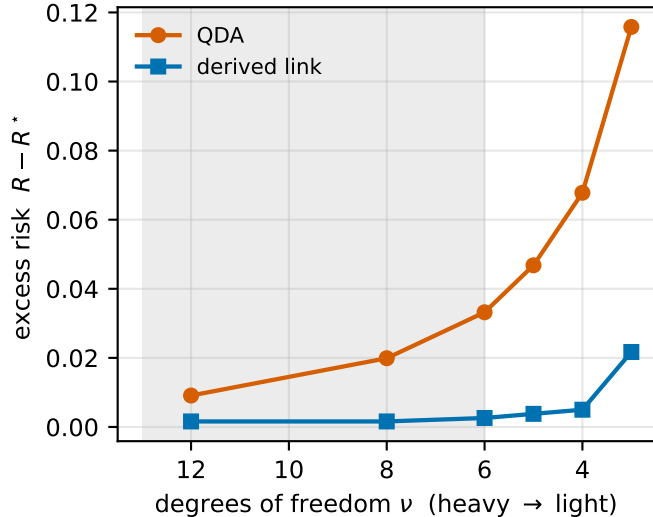
Tail lever ( a = 3 ; shaded = in scope)
