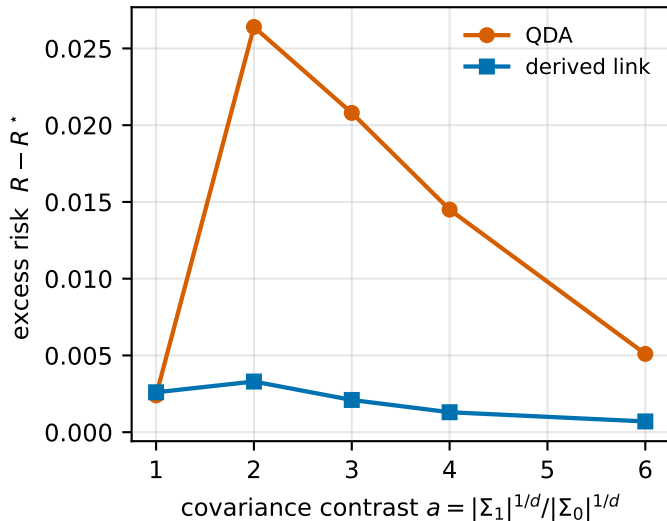
Covariance lever ( \nu = 8 , in scope)
