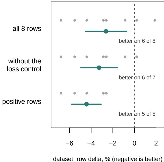
vs best robust statistical baseline
