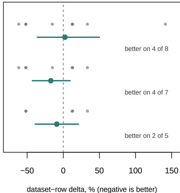
vs best tree ensemble
