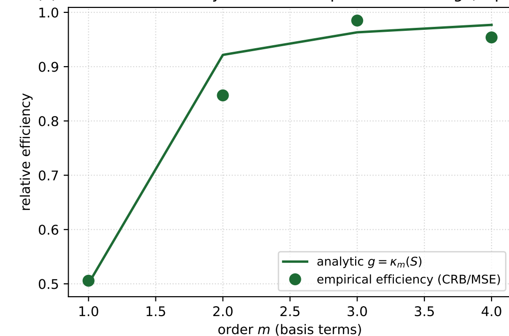
(c) Estimator efficiency tracks the captured fraction g (Laplace)
