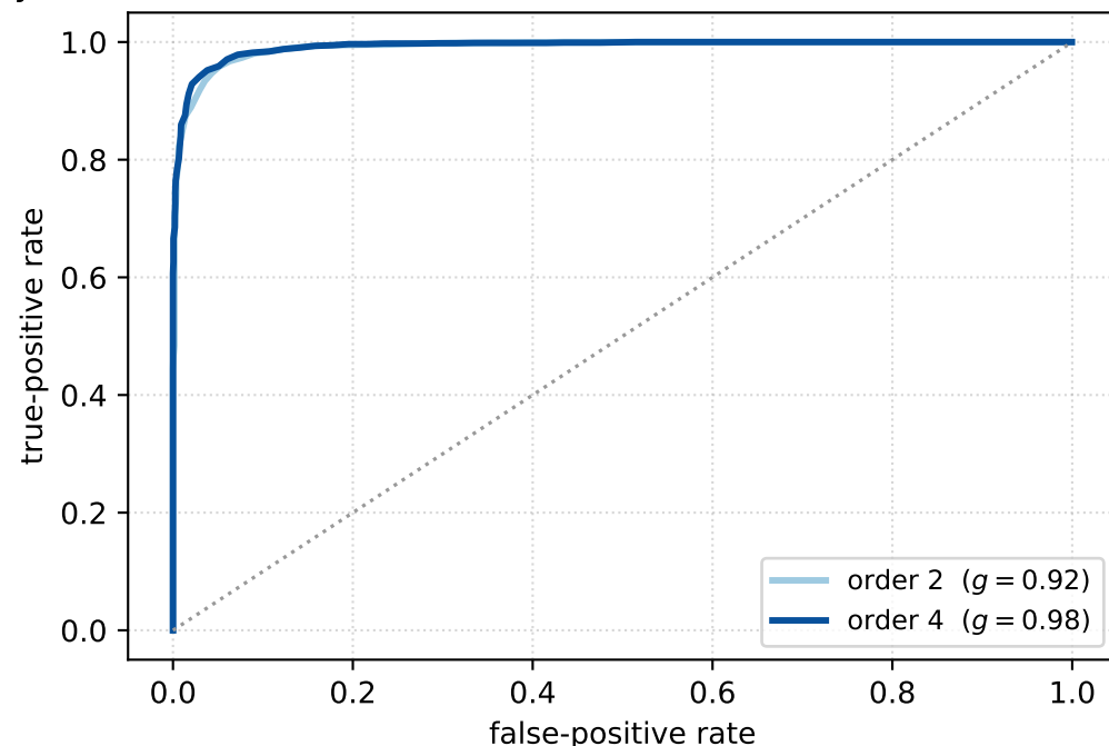
(b) ROC of the order- m projected-score test (Laplace)
