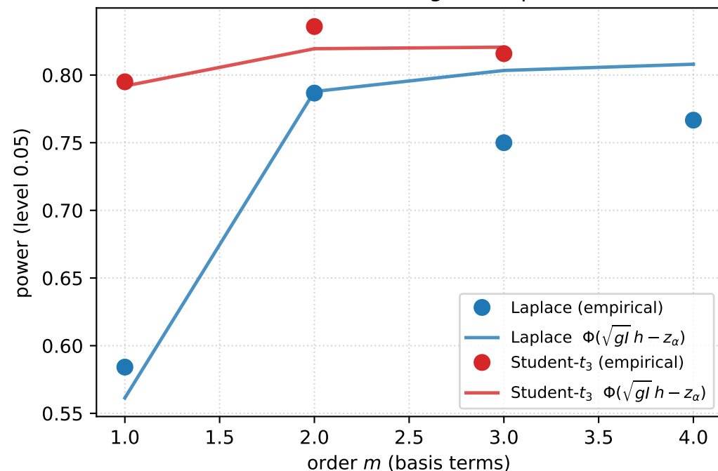
(a) Power rises with order, tracking the captured-fraction theory
