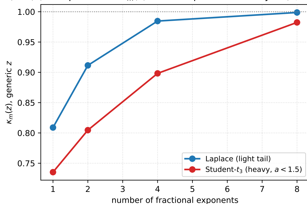
(d) Completeness: \kappa_m(z) \rightarrow 1 as exponents densify in (0, \alpha/2)
