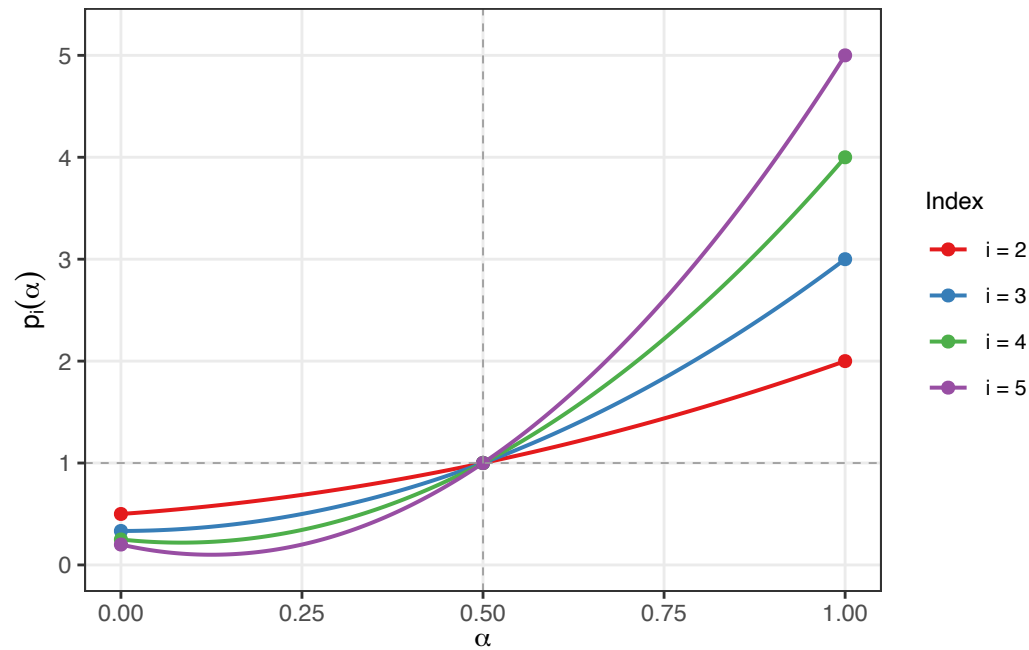
PATP exponent parameterization p_i(\alpha)
