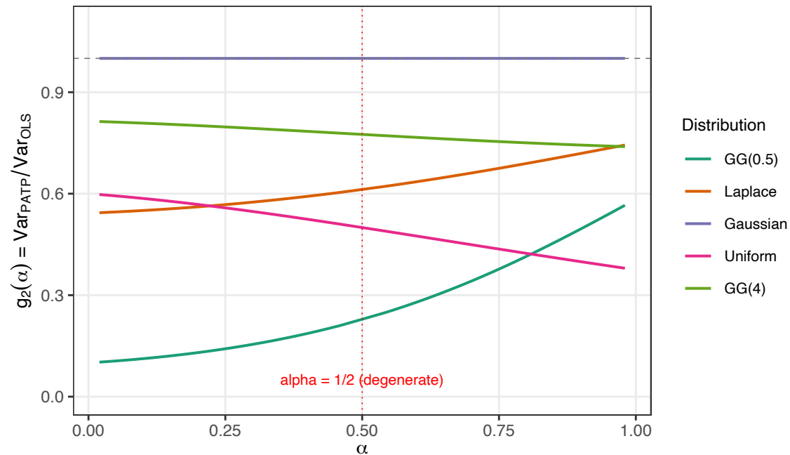
Variance-reduction coefficient g_2(\alpha) for canonical distributions
