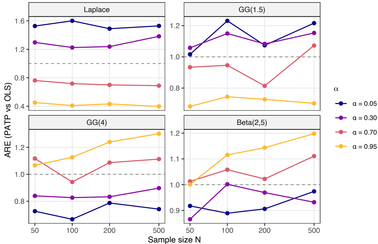
Empirical ARE = \text{Var}_{\text{OLS}}/\text{Var}_{\text{PATP}} over 1000 MC replications
