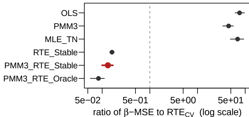
tn1.5: n = 100, \rho = 0.99
