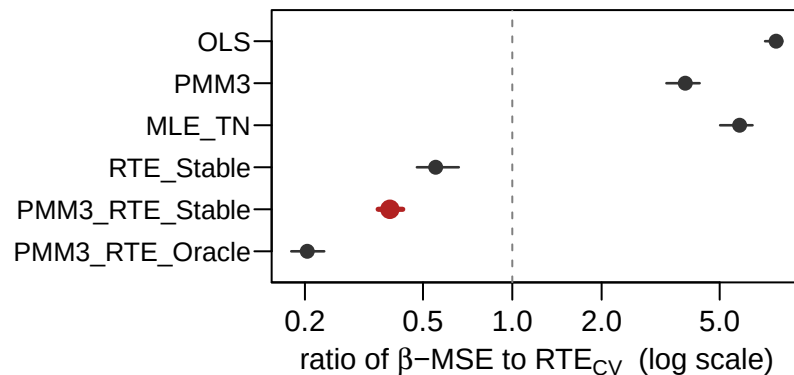
tn1.5: n = 100, \rho = 0.9
