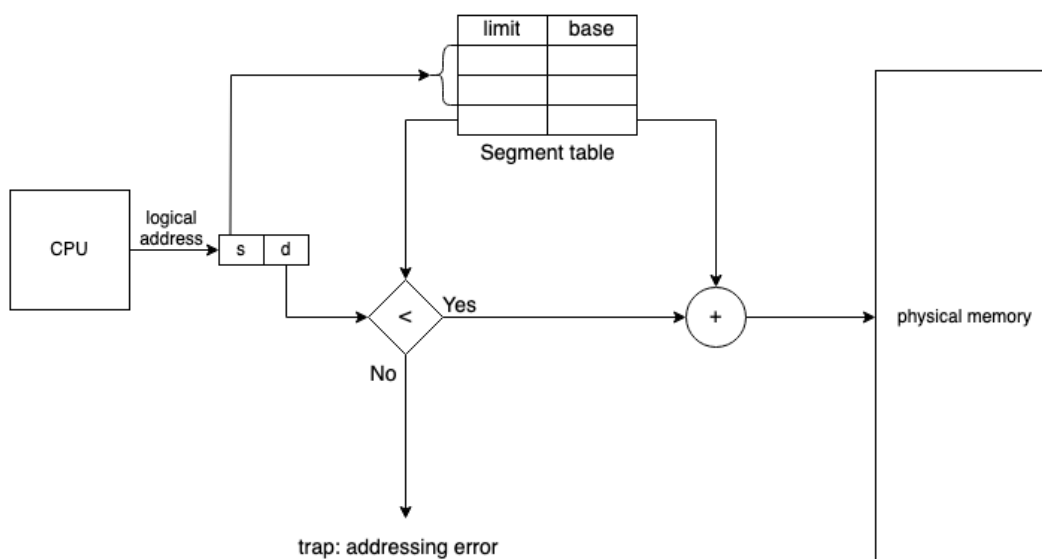
Segmentation hardware
