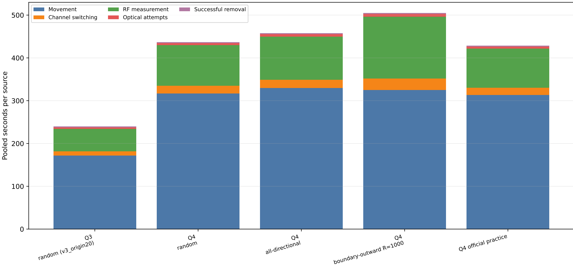
Exact virtual-time decomposition (selected strategies only)
